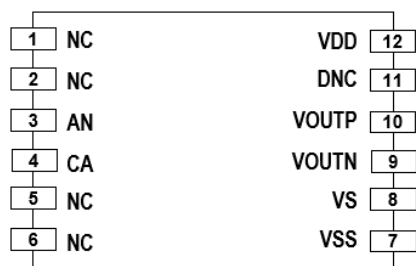
Figure 3: ACFL-3161 Pinouts
