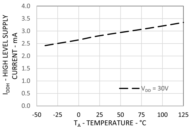
Figure 13: I_{DDH} vs Temperature
