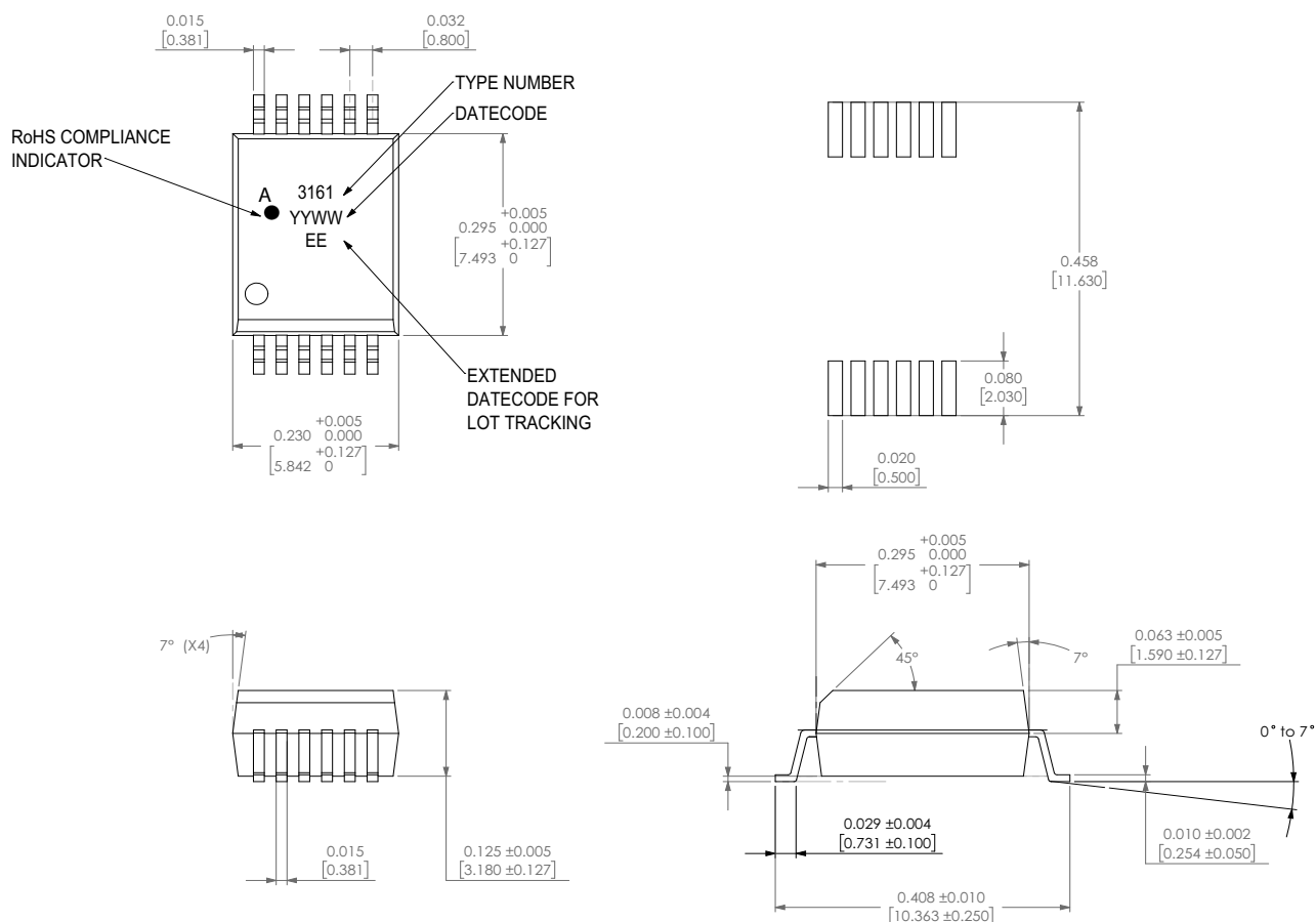
Figure 2: ACFL-3161 Outline Drawing
