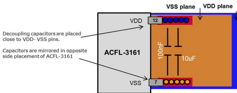
Figure 21: PCB Planes Stack-Up and Bypass Capacitors Placement
