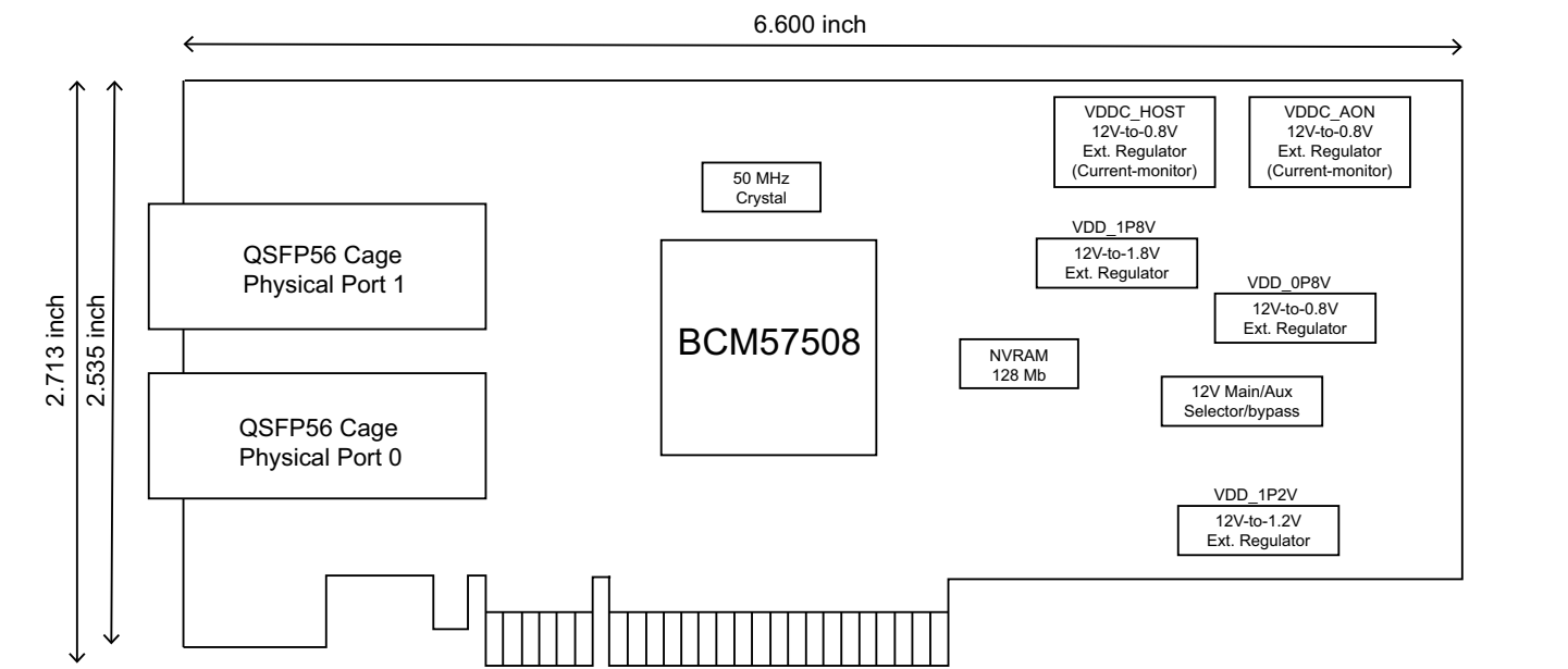
Figure 4: Board Physical Dimensions
