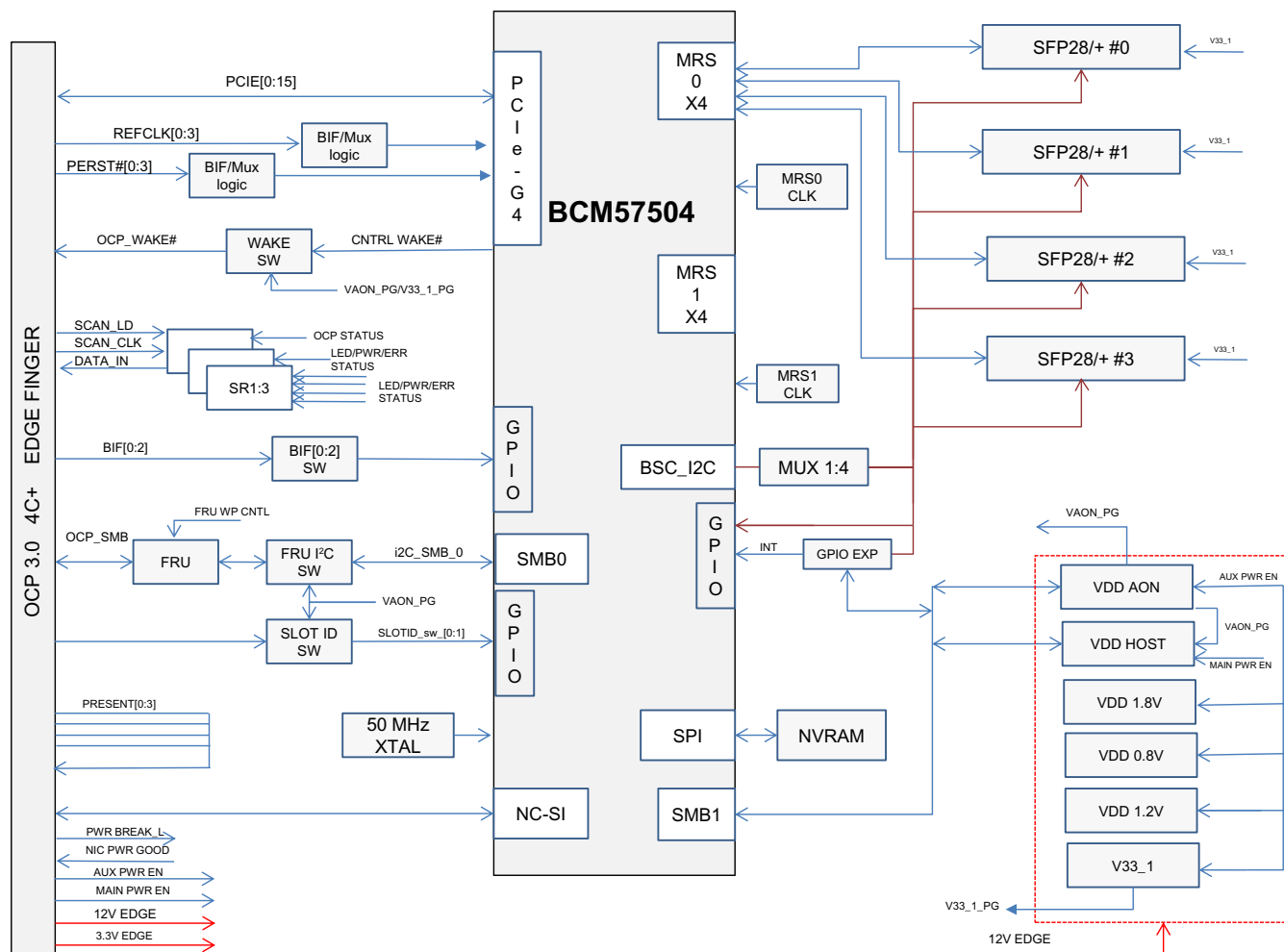
Figure 2: BCM957504-N425G Block Diagram
