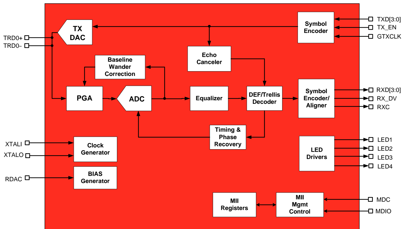
BCM89810 Block Diagram
