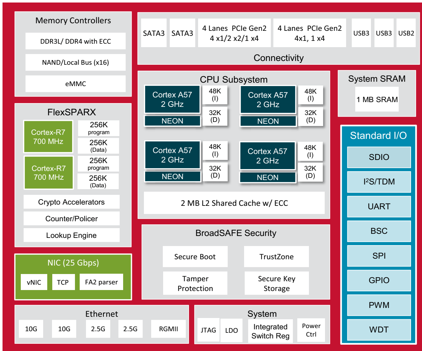
BCM5871X Block Diagram
