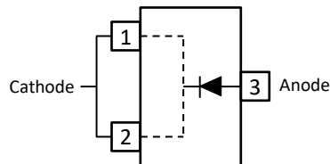
SOT23 Top View
