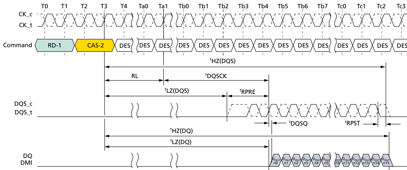
Figure 25: Read Timing
