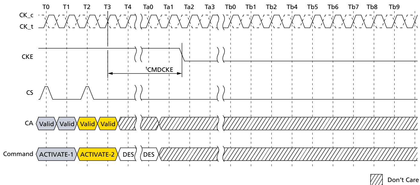
Figure 90: ACTIVATE Command to Power-Down Entry
