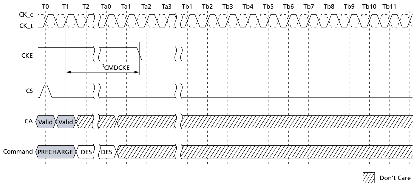
Figure 91: PRECHARGE Command to Power-Down Entry
