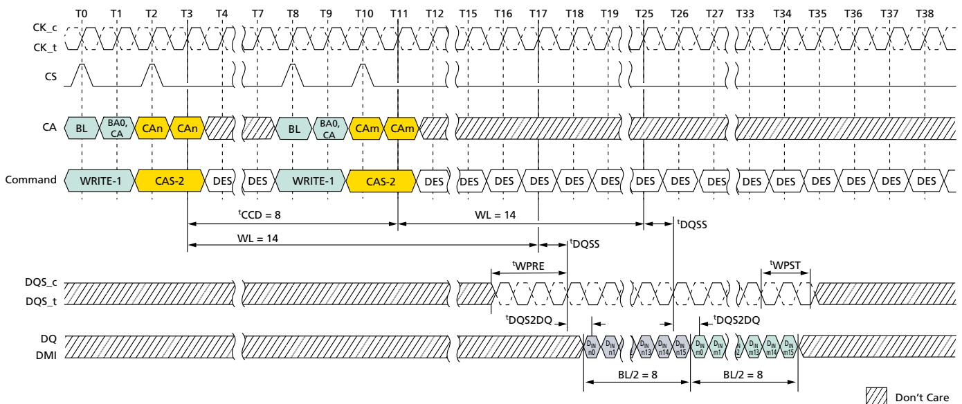
Figure 58: Seamless WRITE: t_{CCD} = \text{MIN} , 1.5nCK Postamble
