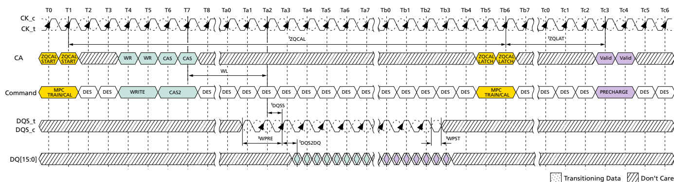
Figure 134: ZQCAL Timing
