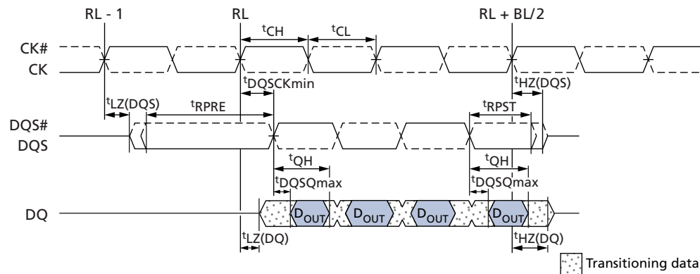
Figure 12: READ Output Timing – t_{DQSCK} (MIN)
