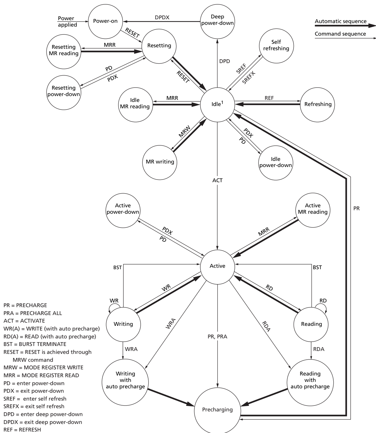
Figure 63: Simplified Bus Interface State Diagram
