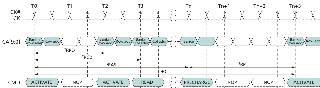
Figure 9: ACTIVATE Command
