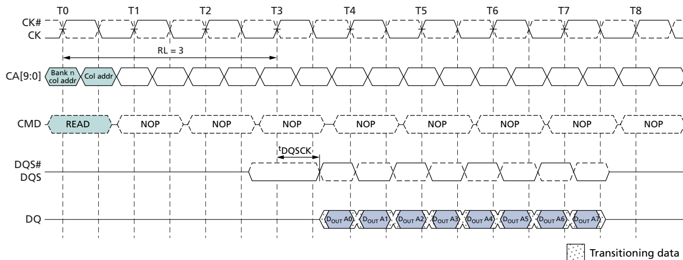
Figure 14: Burst READ – RL = 3, BL = 8, t_{DQSCK} < t_{CK}
