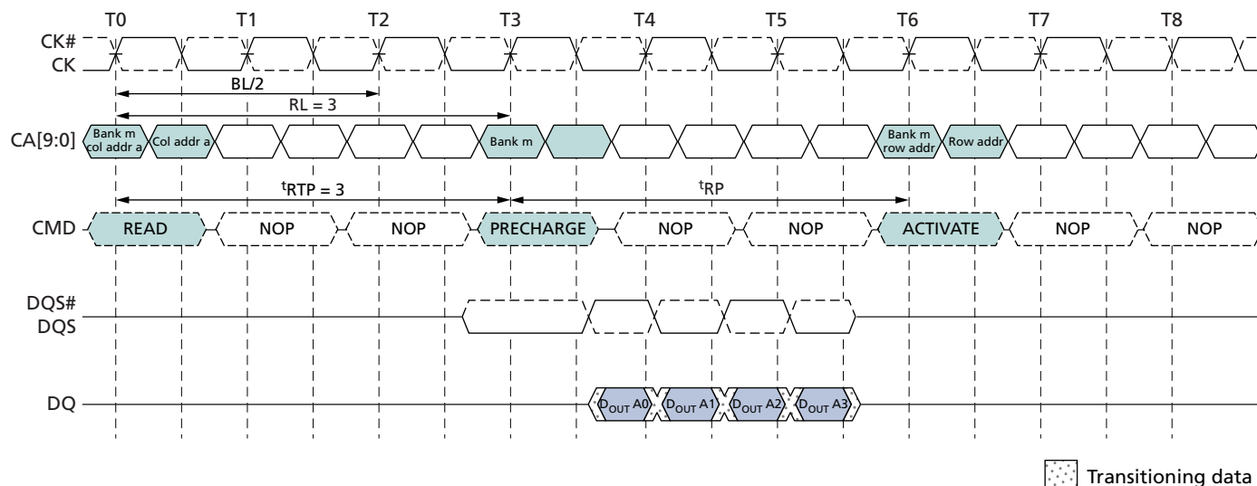
Figure 31: READ Burst Followed by PRECHARGE – RL = 3, BL = 4, RU(t_{RTP}(\text{MIN})/t_{CK}) = 3
