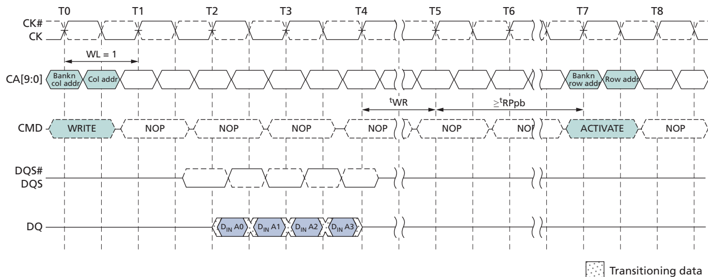
Figure 34: WRITE Burst with Auto Precharge – WL = 1, BL = 4
