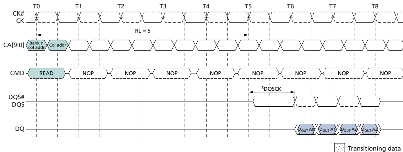
Figure 13: Burst READ – RL = 5, BL = 4, t_{DQSCK} > t_{CK}
