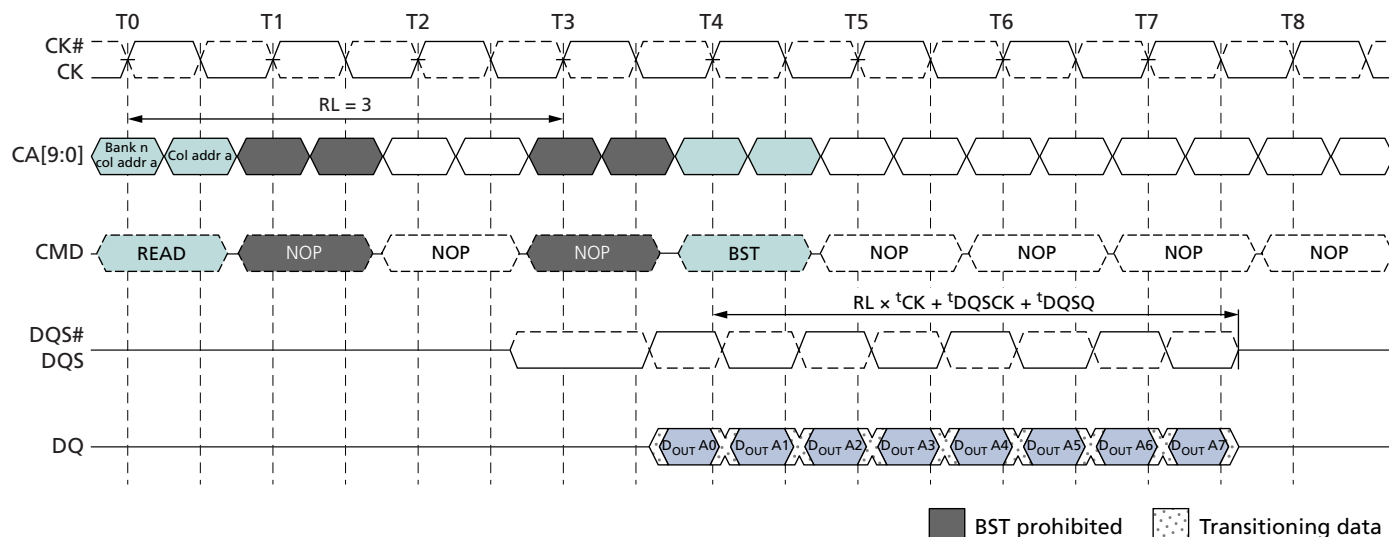
Figure 27: Burst READ Truncated by BST – RL = 3, BL = 16
