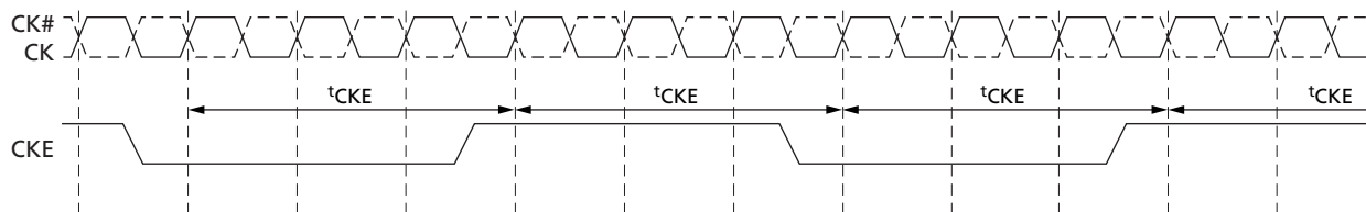
Figure 51: CKE Intensive Environment
