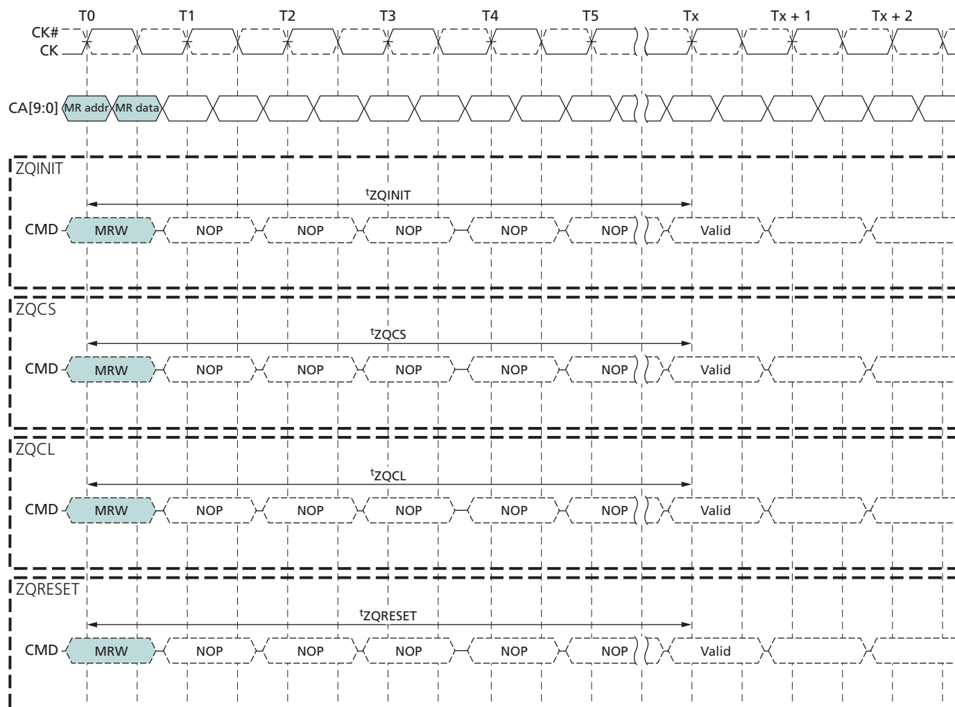
Figure 49: ZQ Timings
