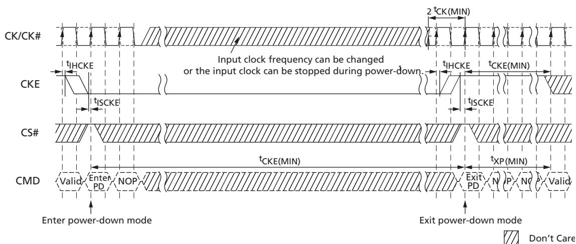
Figure 50: Power-Down Entry and Exit Timing
