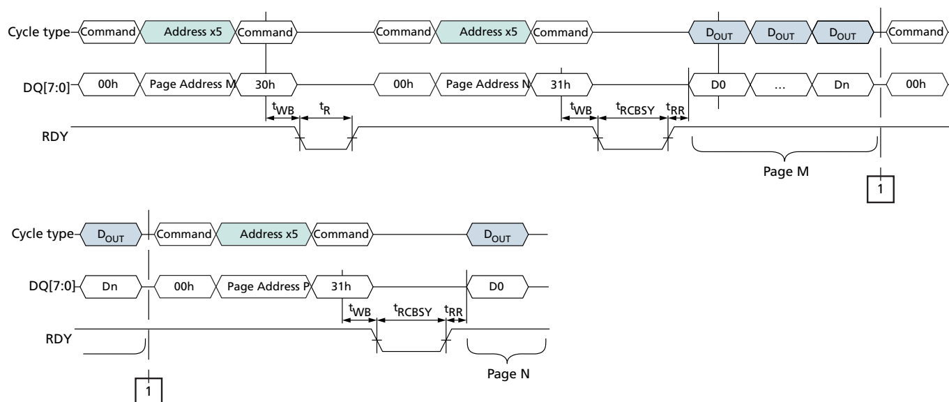
Figure 55: READ PAGE CACHE RANDOM (00h-31h) Operation
