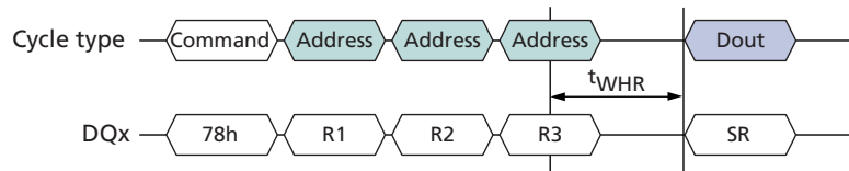
Figure 48: READ STATUS ENHANCED (78h) Operation
