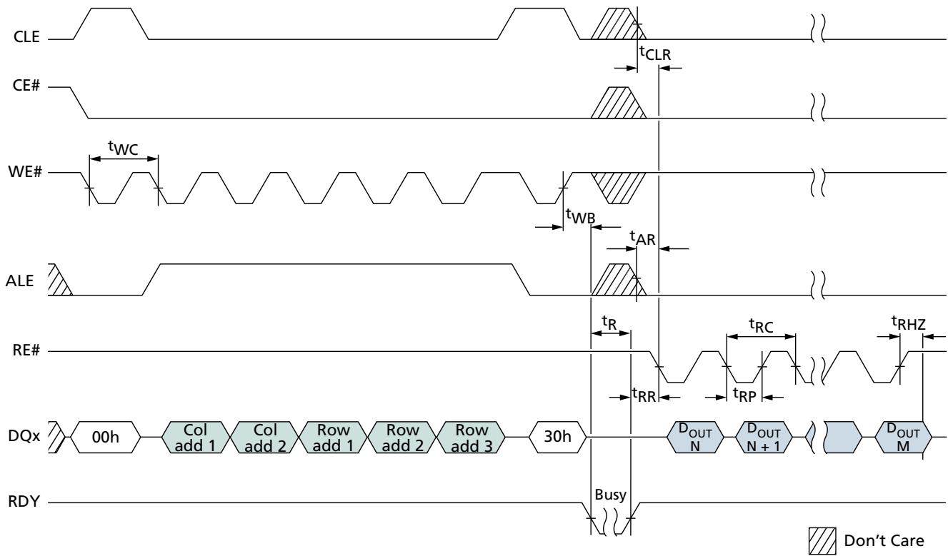
Figure 79: READ PAGE
