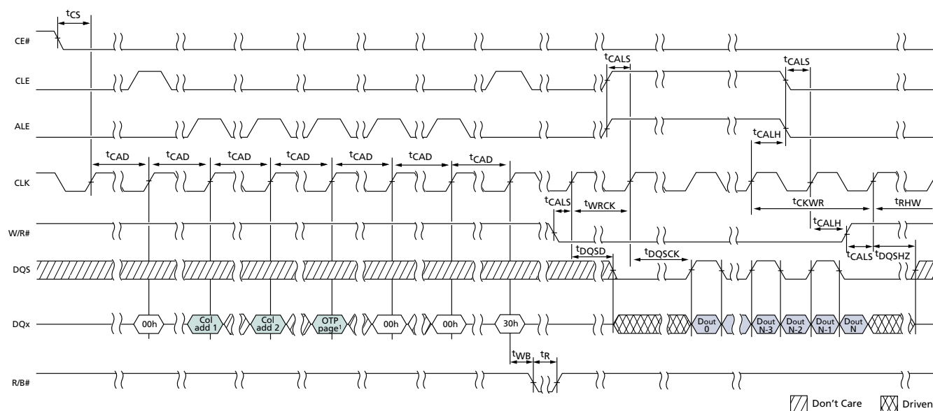
Figure 115: READ OTP PAGE
