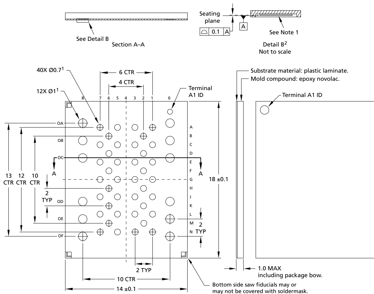
Figure 6: 52-Pad VLGA
