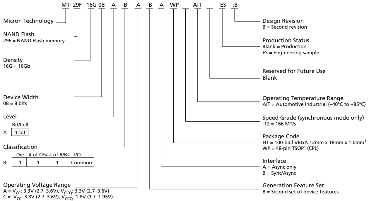
Figure 1: Part Numbering
