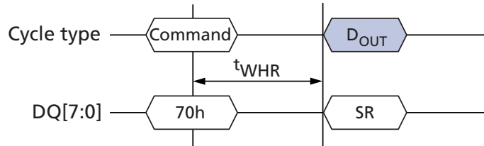
Figure 47: READ STATUS (70h) Operation
