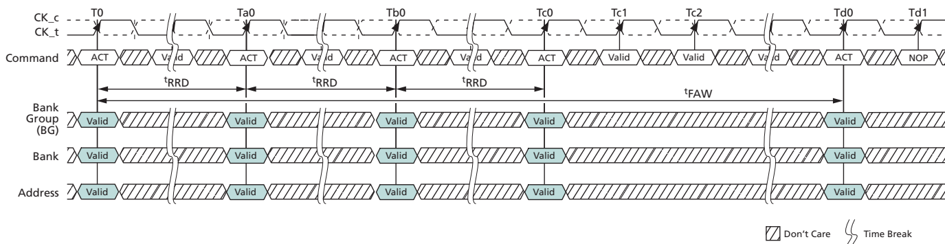
Figure 79: t_{FAW} Timing
