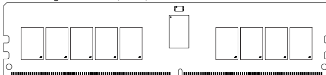
Figure 1: 288-Pin RDIMM (MO-309, R/C-E1, R/C-E2)
