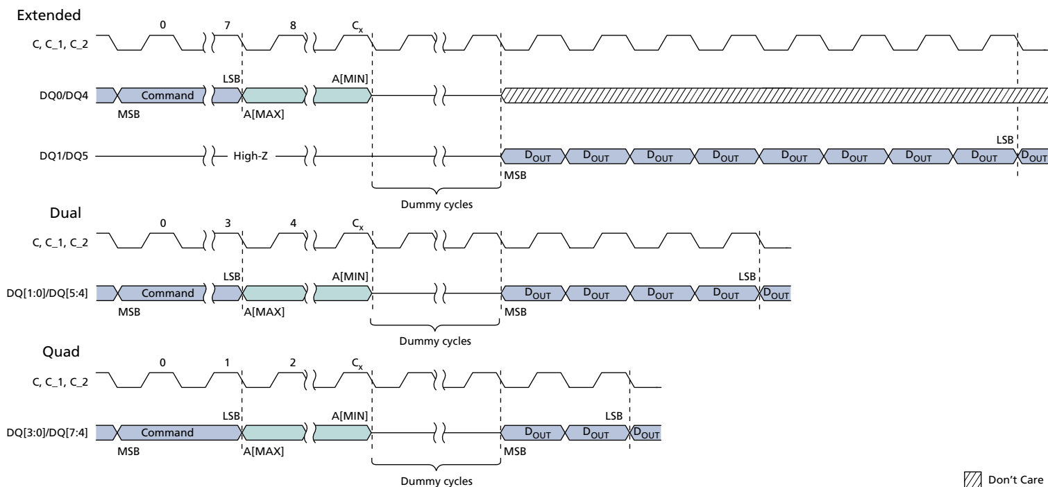
Figure 17: READ SERIAL FLASH DISCOVERY PARAMETER Command – 5Ah
