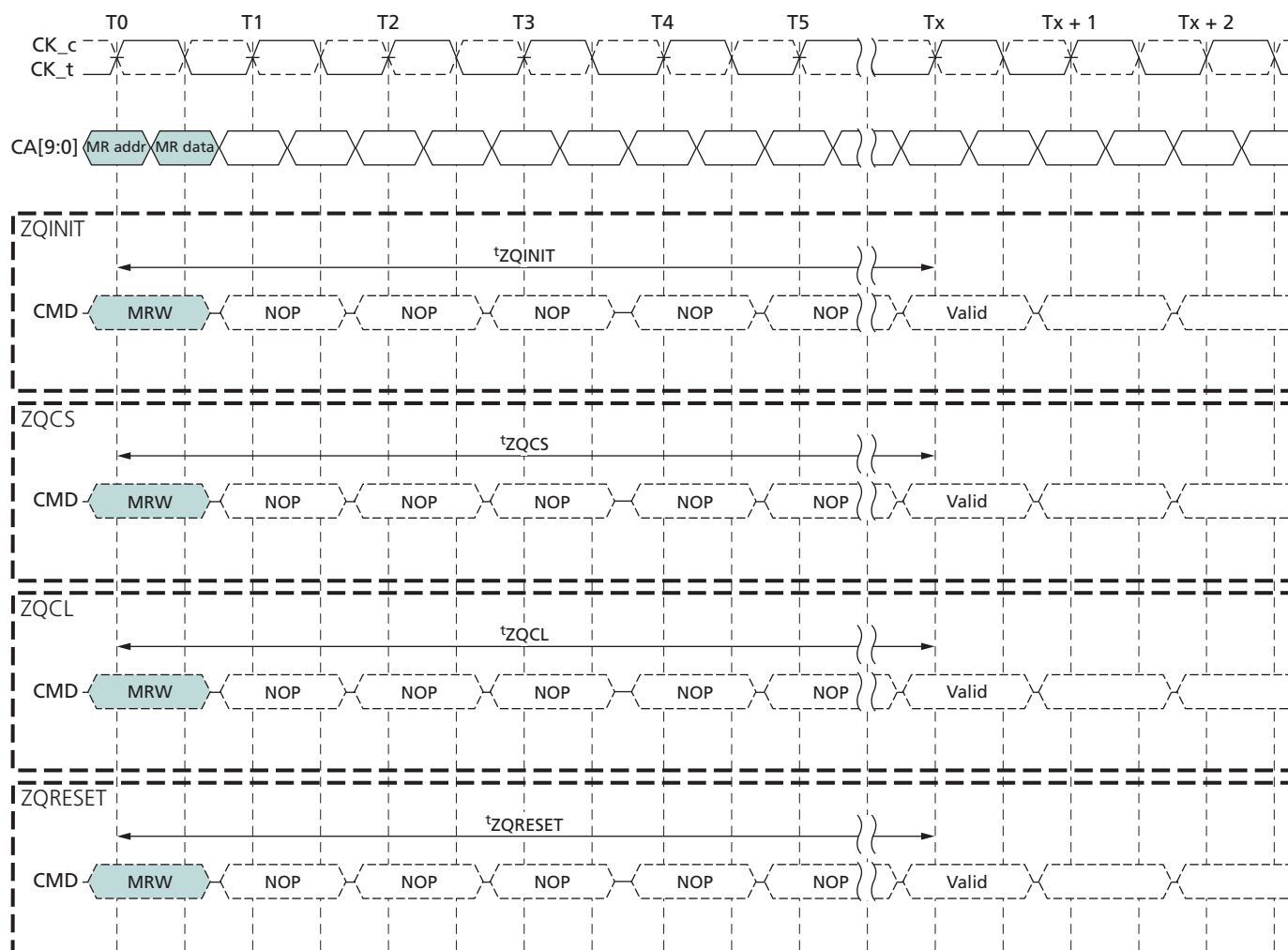
Figure 49: ZQ Timings
