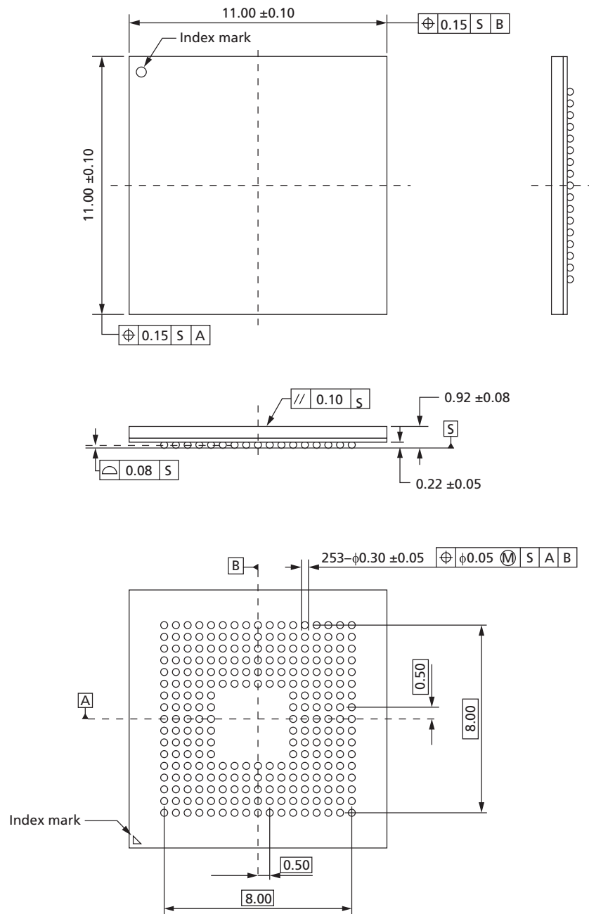
Figure 7: 253-Ball FBGA (11mm x 11mm) – EDFA164A2MA
