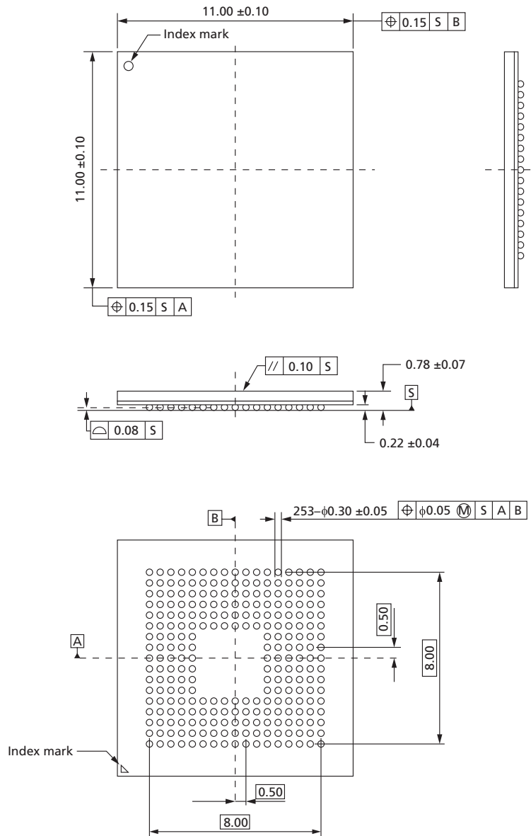
Figure 6: 253-Ball FBGA (11mm x 11mm) – EDF8164A3MA
