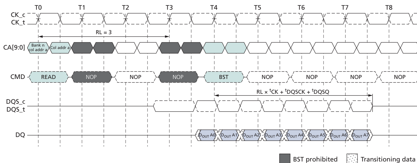
Figure 28: Burst READ Truncated by BST – RL = 3, BL = 16
