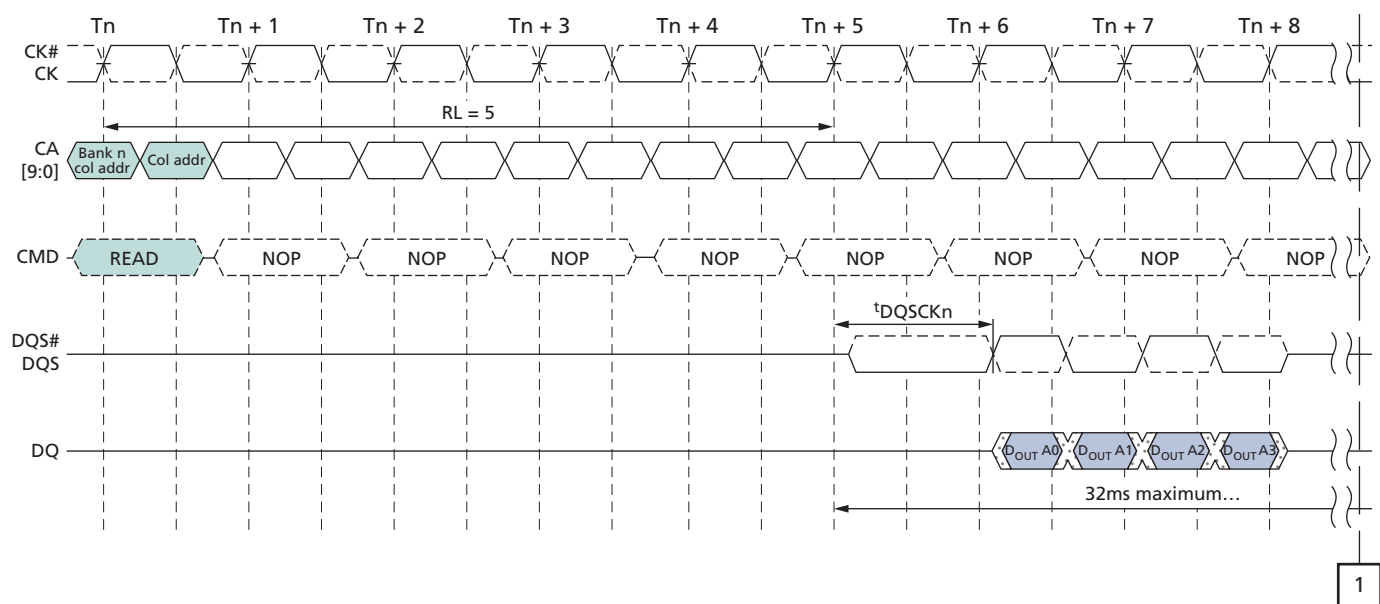
Figure 16: t_{DQSKDL} Timing
