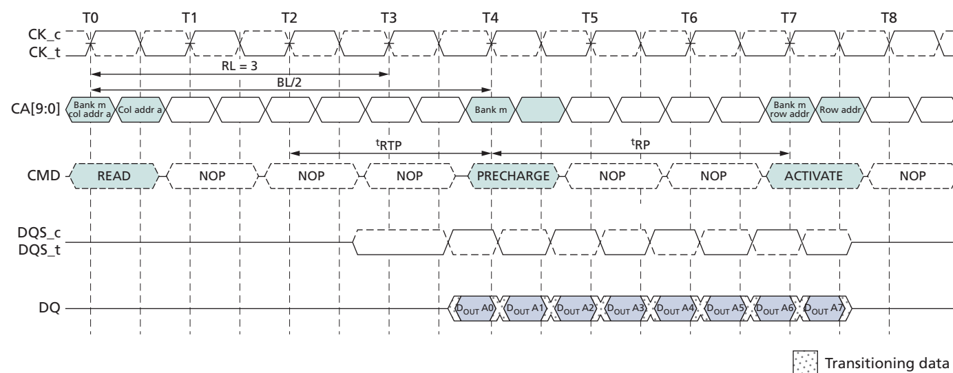
Figure 31: READ Burst Followed by PRECHARGE – RL = 3, BL = 8, RU(t_{RTP}(\text{MIN})/t_{CK}) = 2
