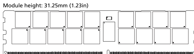
Figure 2: 288-Pin LRDIMM (MO-309, R/C-E2)
