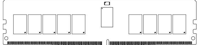
Figure 1: 288-Pin RDIMM (MO-309, R/C-E1, R/C-E2)
