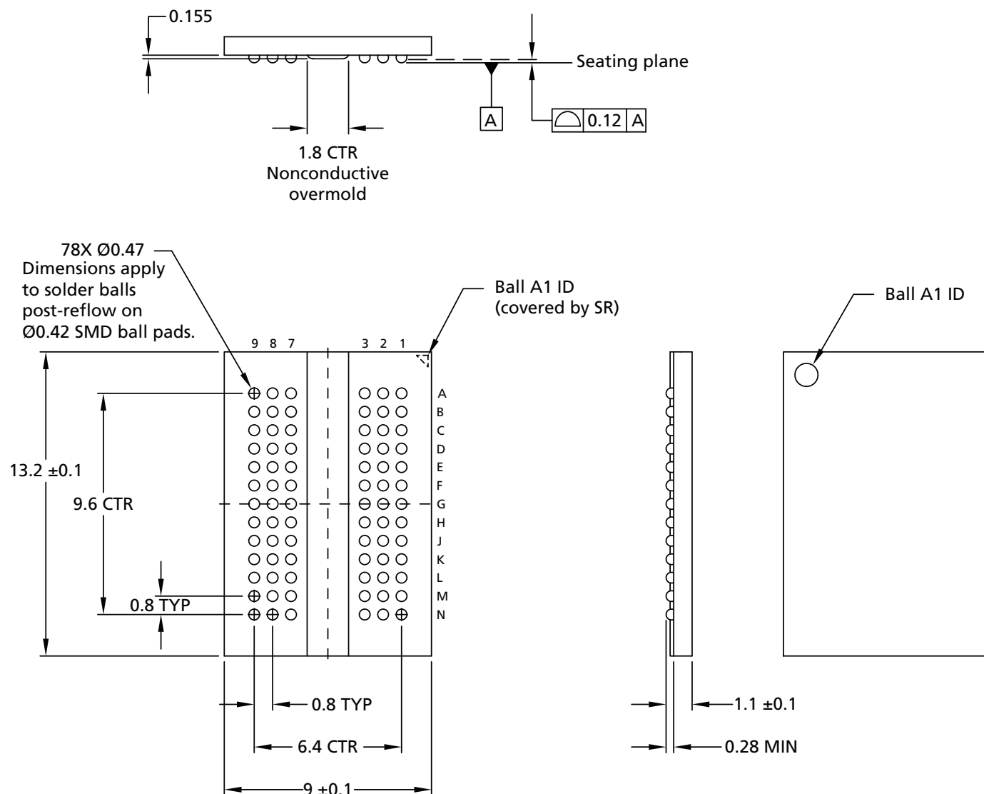
Figure 7: 78-Ball FBGA – x4, x8 (PM)
