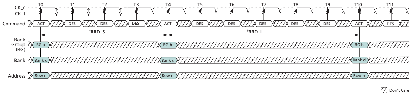
Figure 122: t_{RRD} Timing
