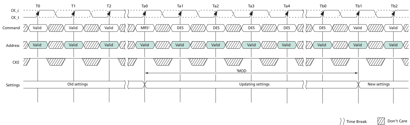
Figure 18: t_{MOD} Timing
