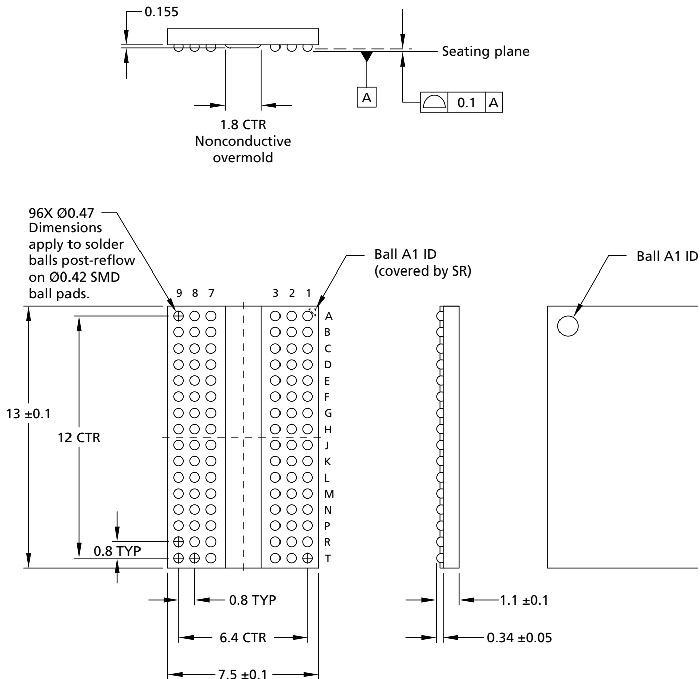
Figure 13: 96-Ball FBGA – x16 (TB)
