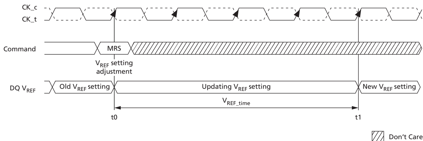
Figure 67: V_{\text{REFDQ}} Timing Diagram for V_{\text{REF,time}} Parameter
