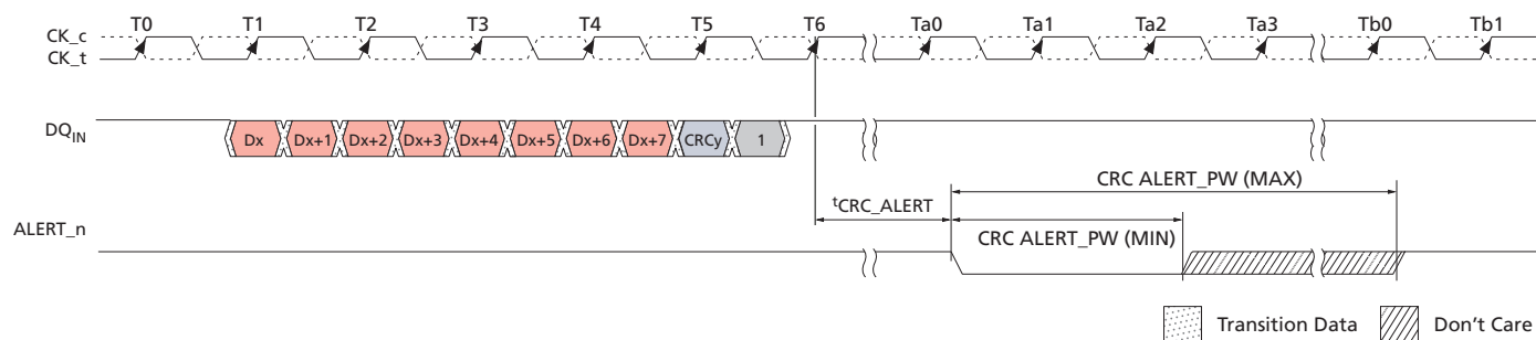
Figure 109: CRC Error Reporting
