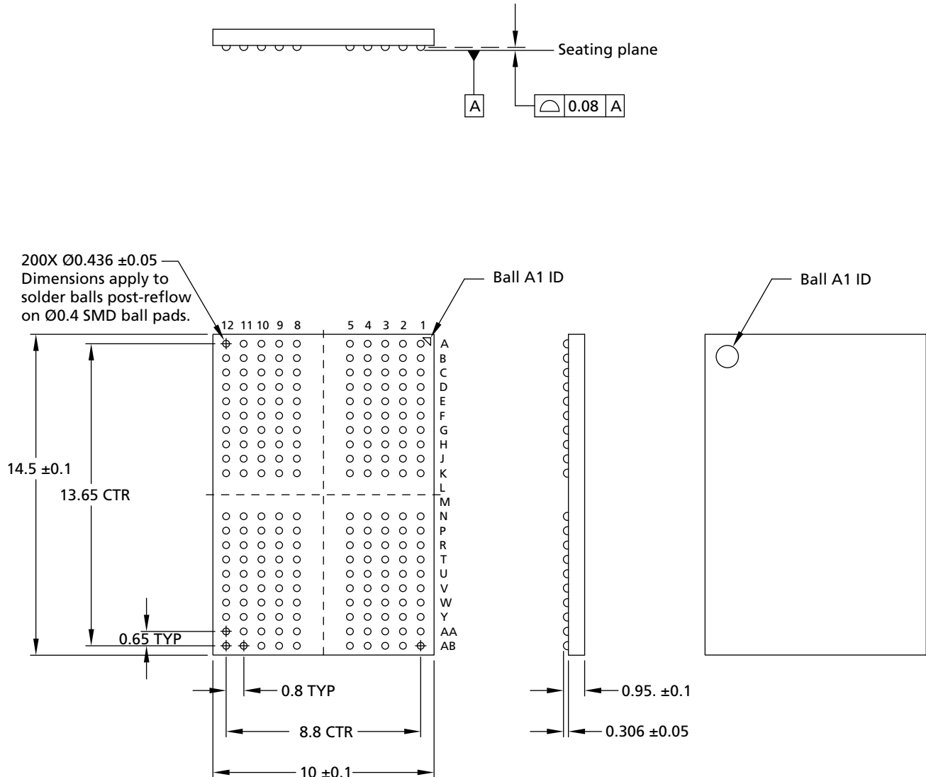
Figure 9: 200-Ball TFBGA – 10mm x 14.5mm x 1.05mm (Package Code: ZW)
