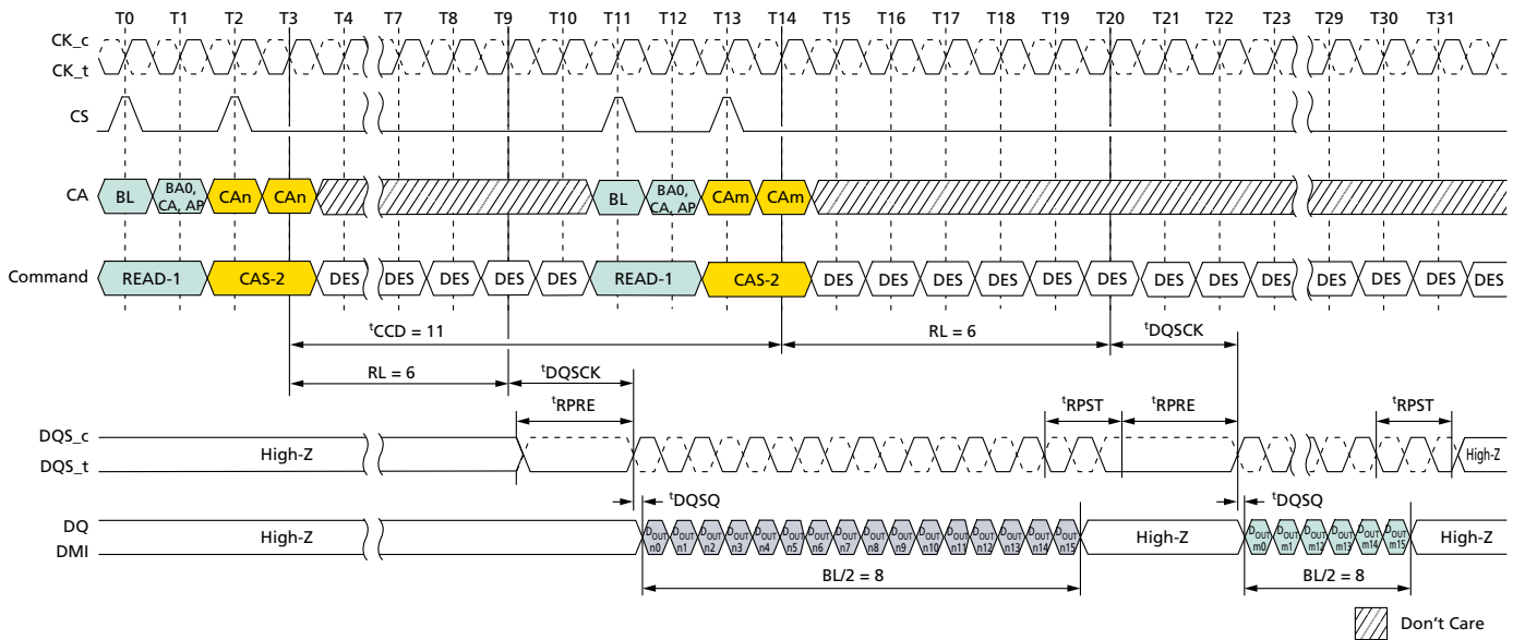
Figure 54: Consecutive READ: t_{CCD} = \text{MIN} + 3 , Preamble = Static, 1.5n\text{CK} Postamble
