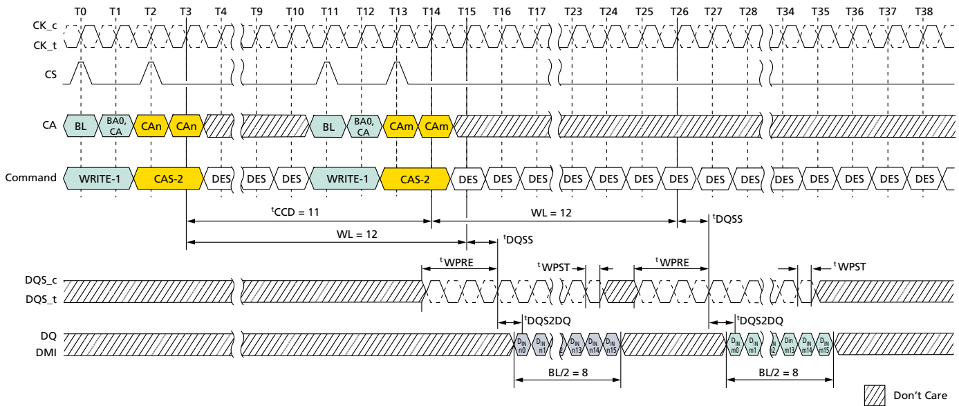
Figure 63: Consecutive WRITE: t_{CCD} = \text{MIN} + 3, 0.5n\text{CK} Postamble
