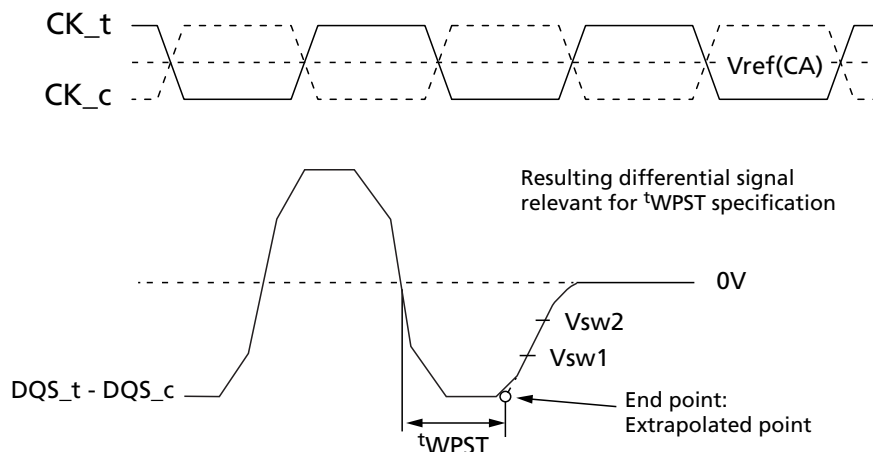
Figure 34: Method for Calculating t_{WPST} Transitions and Endpoints
