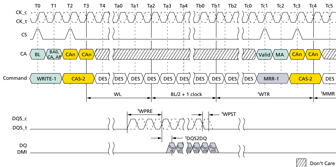
Figure 97: WRITE-to-MRR Timing
