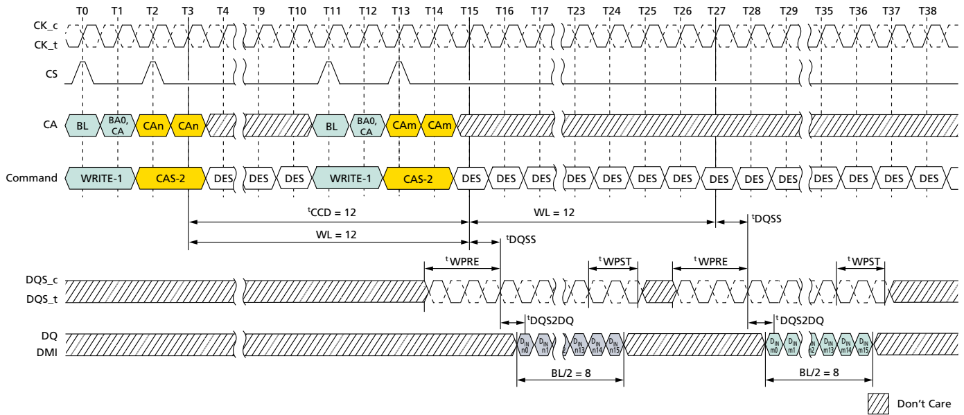
Figure 65: Consecutive WRITE: t_{CCD} = \text{MIN} + 4, 1.5n\text{CK} Postamble
