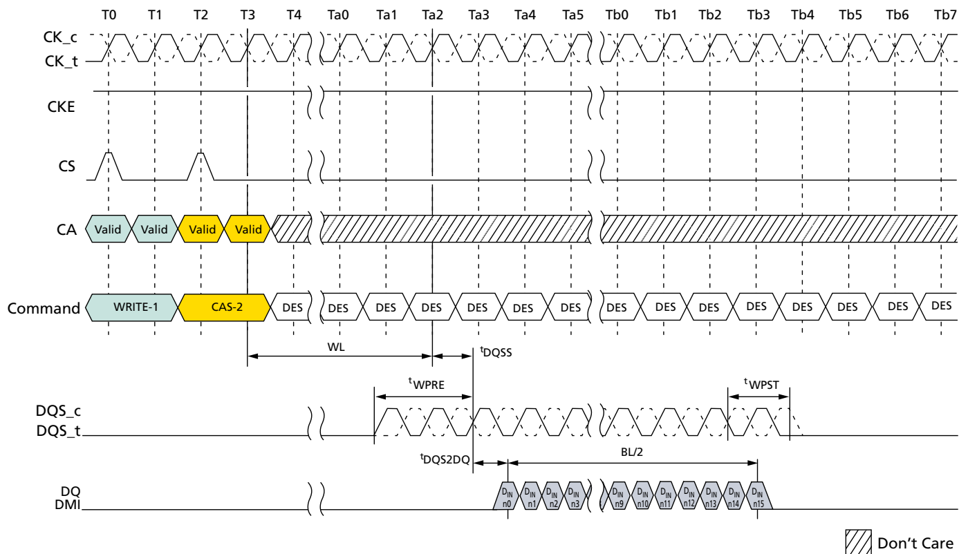
Figure 21: DQS Write Preamble and Postamble – 1.5nCK Postamble
