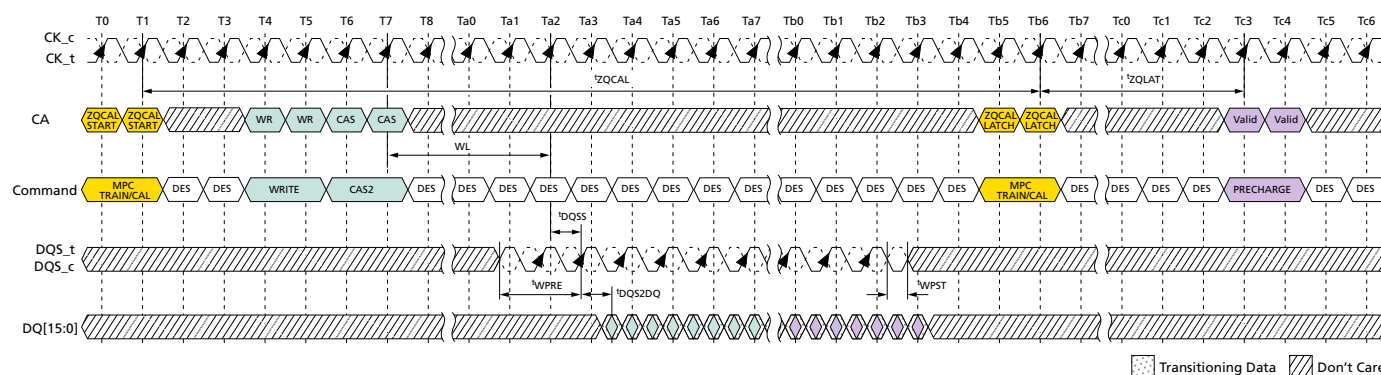
Figure 139: ZQCAL Timing
