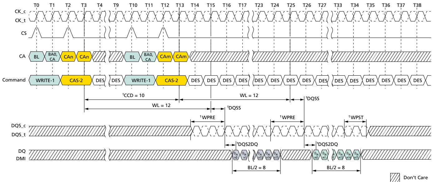
Figure 62: Consecutive WRITE: t_{CCD} = \text{MIN} + 2, 1.5n\text{CK} Postamble
