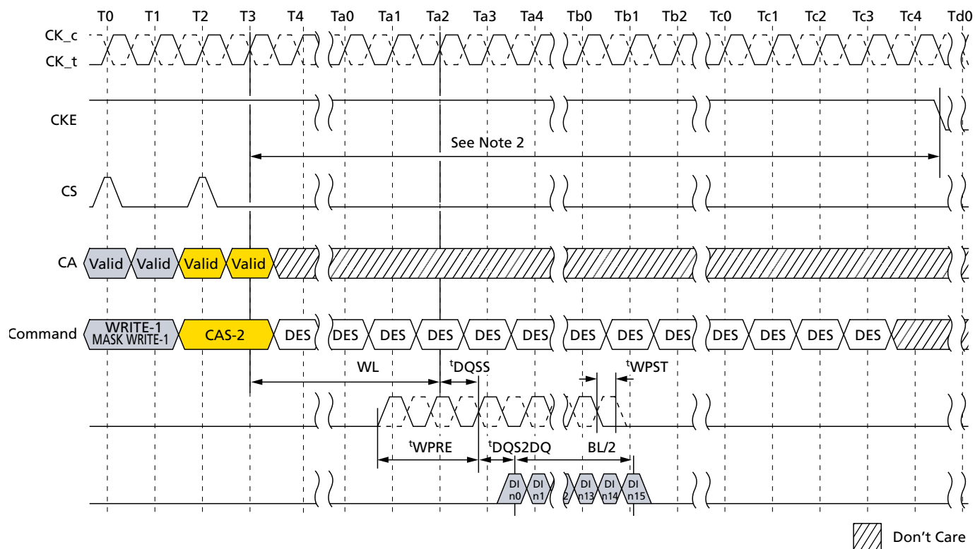
Figure 88: Write With Auto Precharge and Mask Write With Auto Precharge to Power-Down Entry
