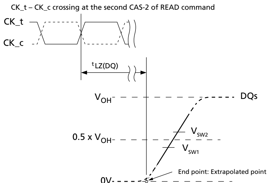
Figure 184: t_{LZ}(DQ) Method for Calculating Transitions and Endpoint
