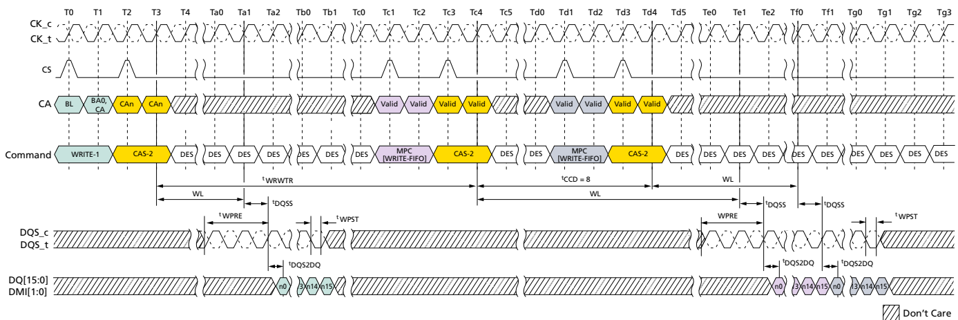
Figure 124: WRITE-FIFO – t_{WPRE} = 2nCK , t_{WPST} = 0.5nCK
