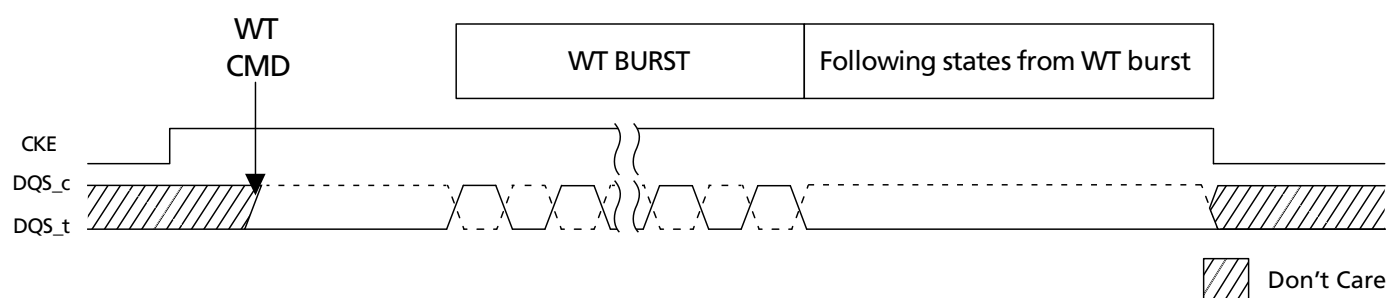
Figure 39: WDQS Control Mode 1
