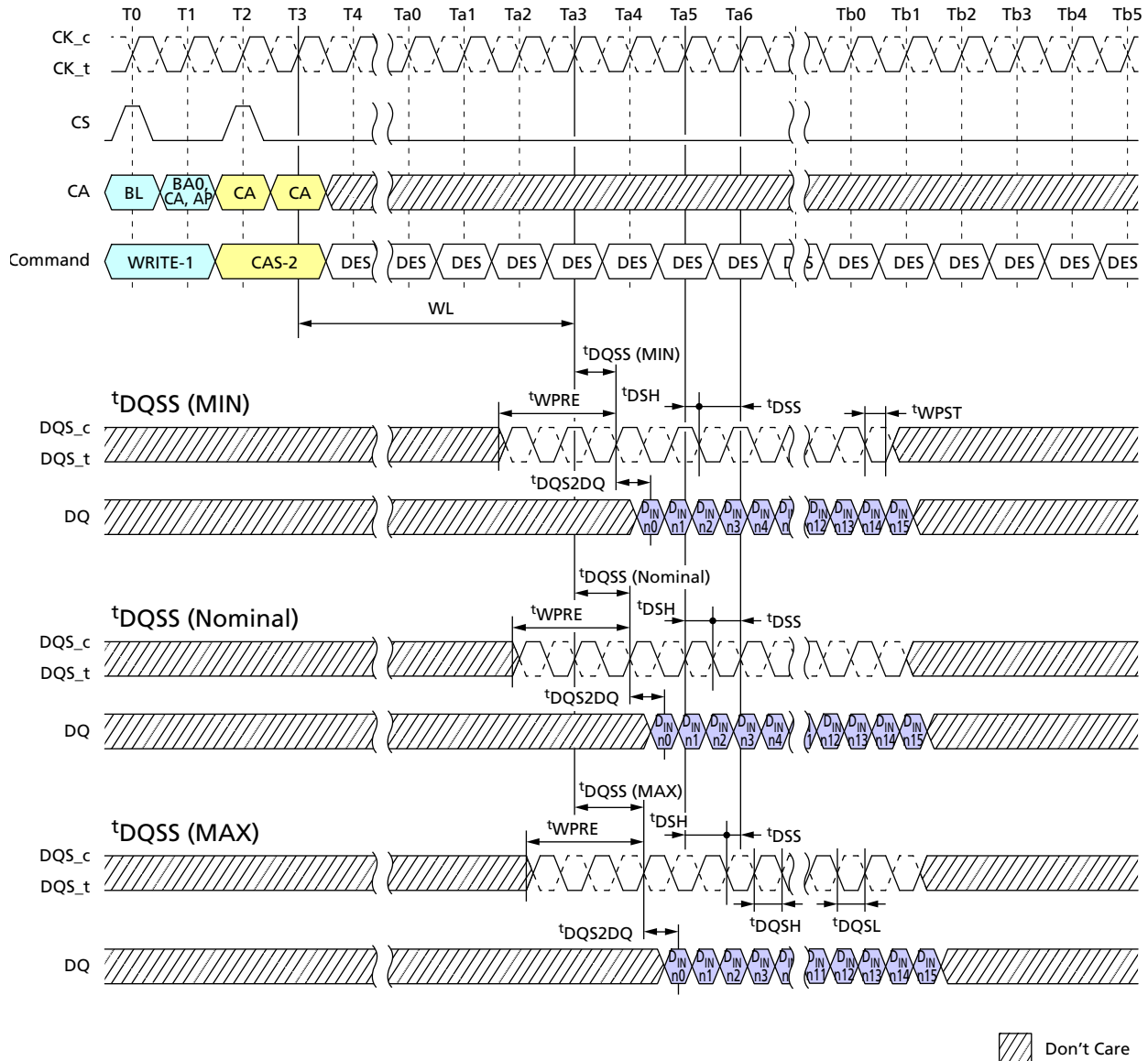
Figure 32: Write Timing
