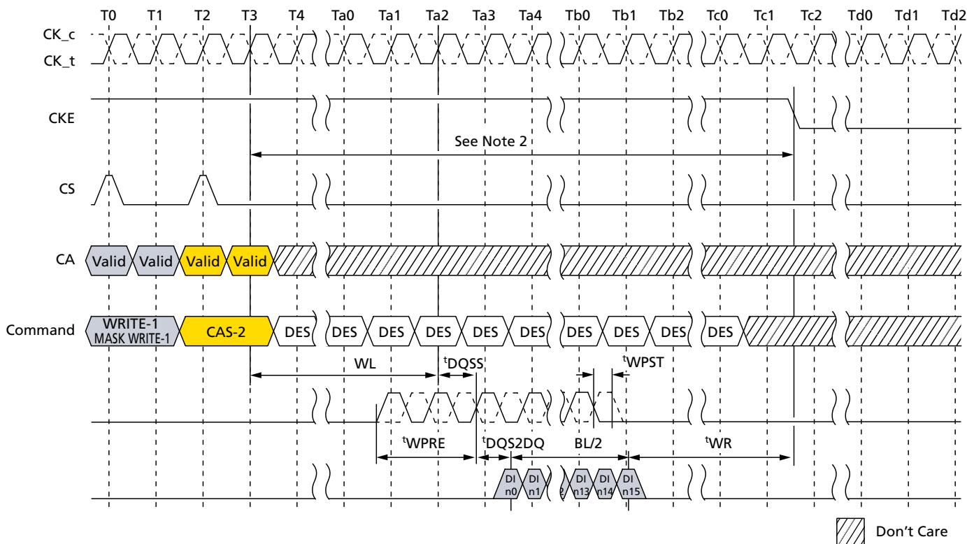
Figure 87: Write and Mask Write to Power-Down Entry
