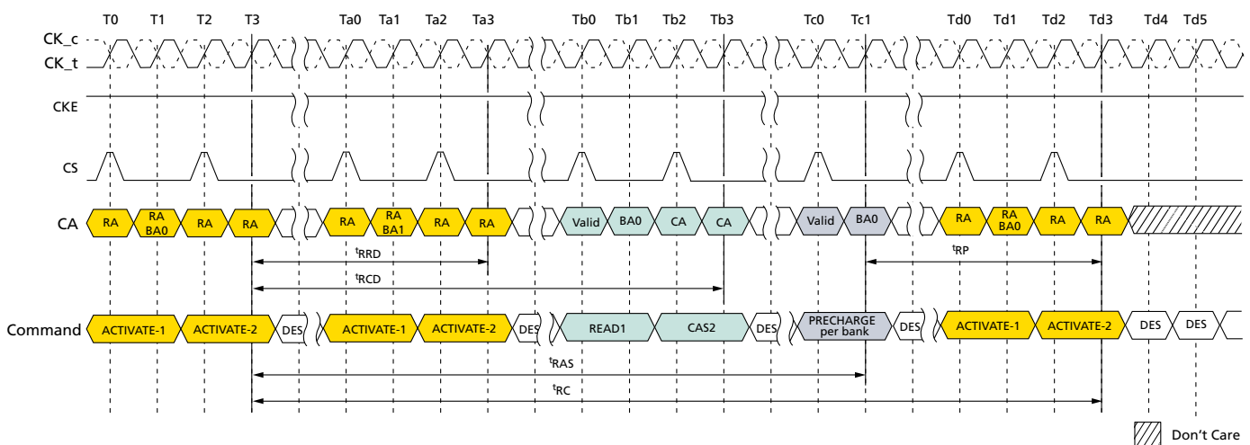
Figure 16: ACTIVATE Command
