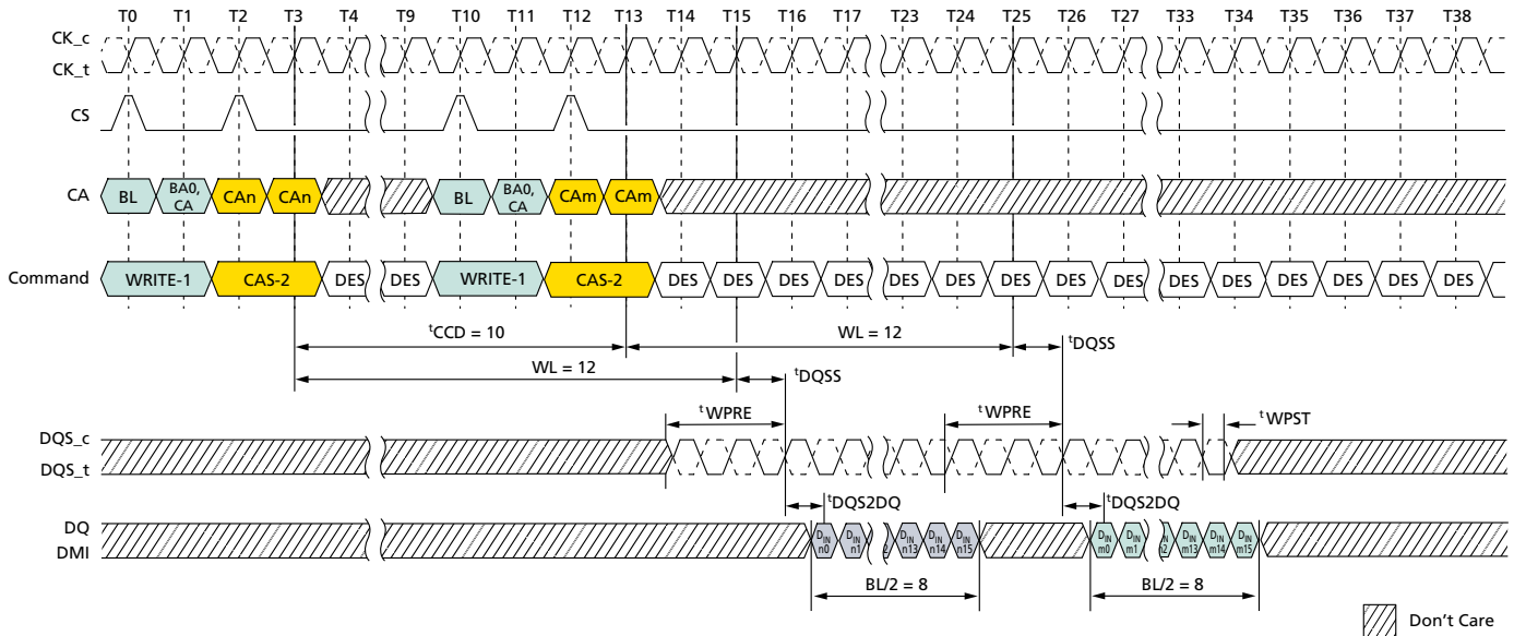
Figure 61: Consecutive WRITE: t_{CCD} = \text{MIN} + 2, 0.5n\text{CK} Postamble
