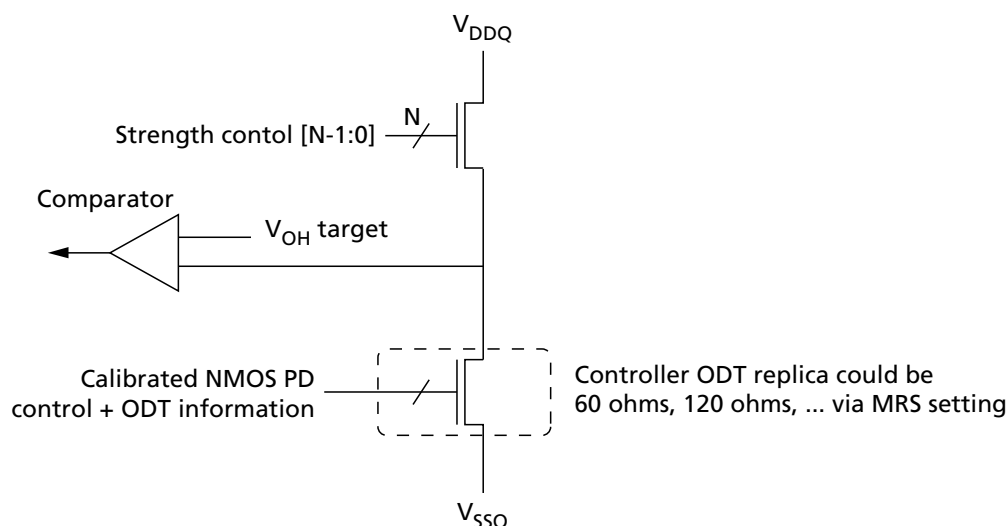
Figure 191: Pull-Up Calibration
