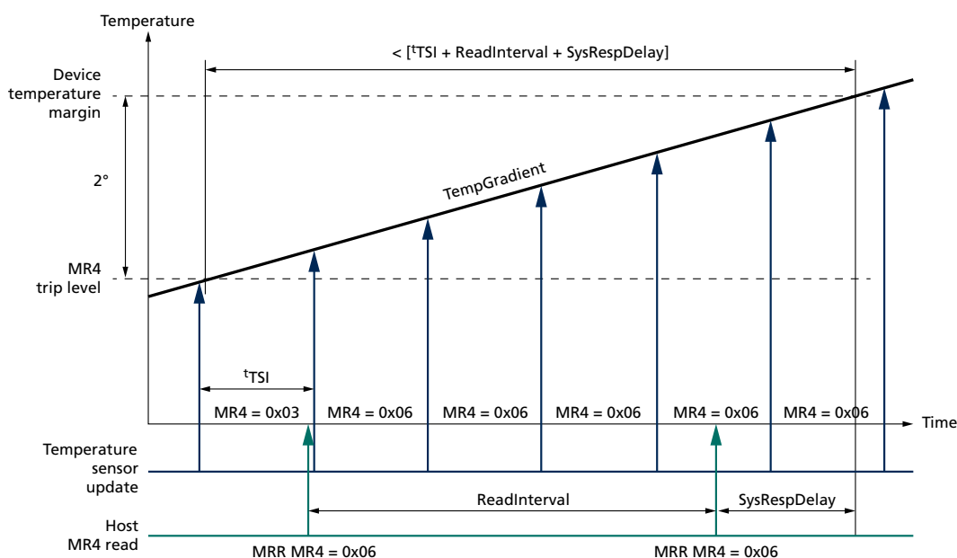
Figure 138: Temperature Sensor Timing
