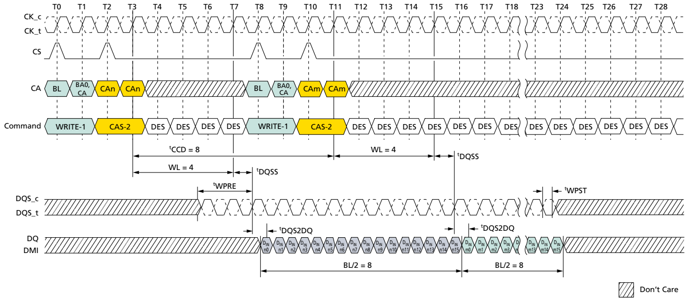
Figure 56: Seamless WRITE: t_{CCD} = \text{MIN}, 0.5nCK Postamble
