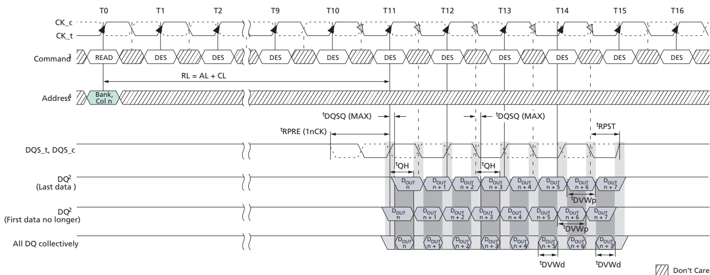
Figure 127: Data Strobe-to-Data Relationship
