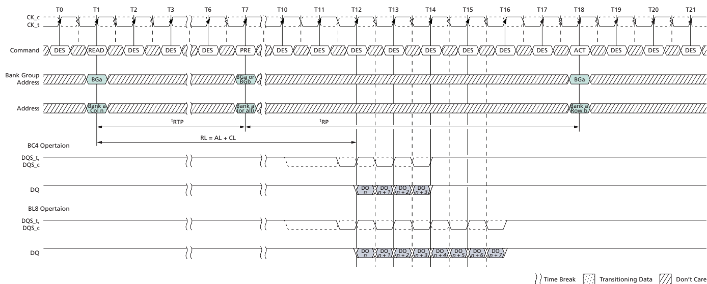
Figure 154: READ to PRECHARGE with 2 t CK Preamble
