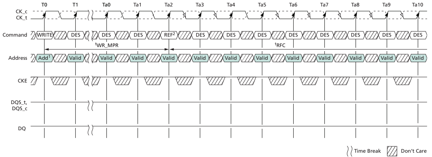
Figure 43: WRITE-to-REFRESH Timing
