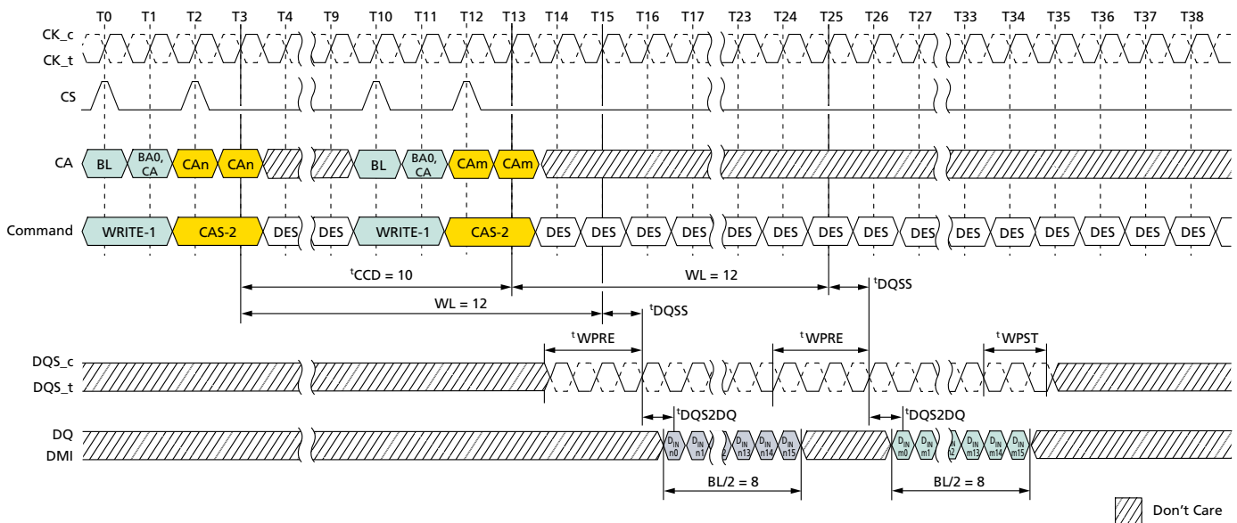
Figure 62: Consecutive WRITE: t_{CCD} = \text{MIN} + 2, 1.5n\text{CK} Postamble
