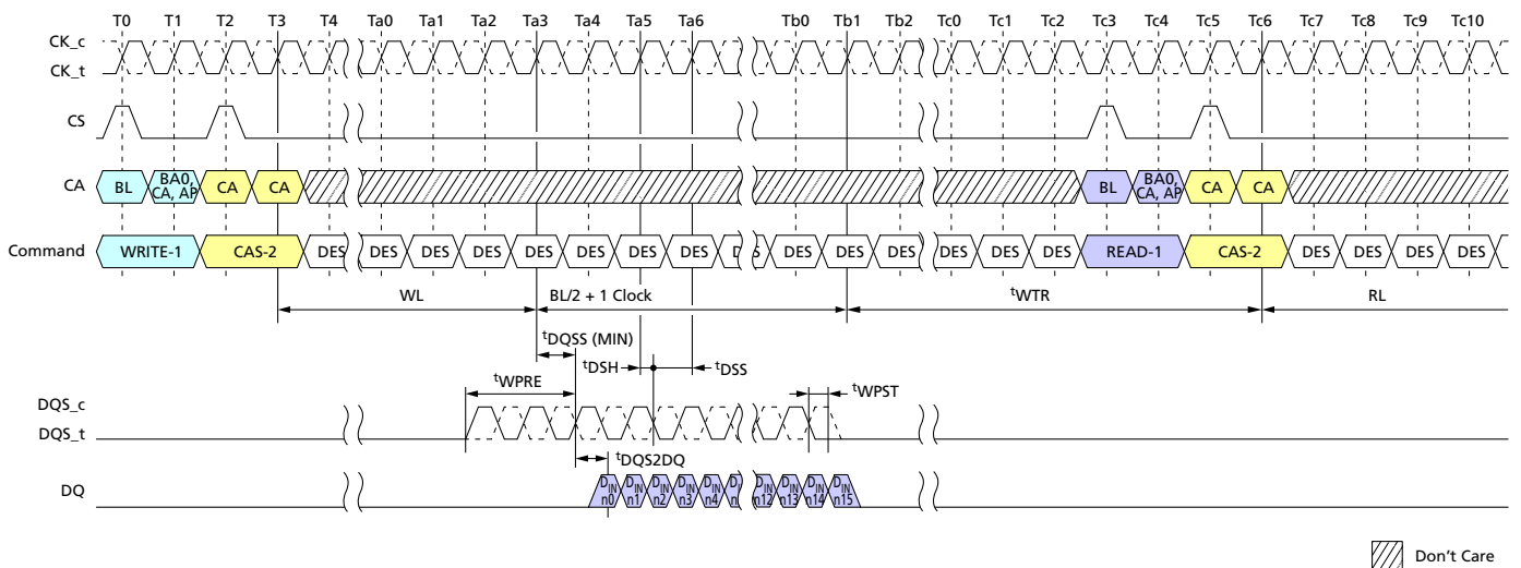
Figure 31: Burst Write Followed by Burst Read
