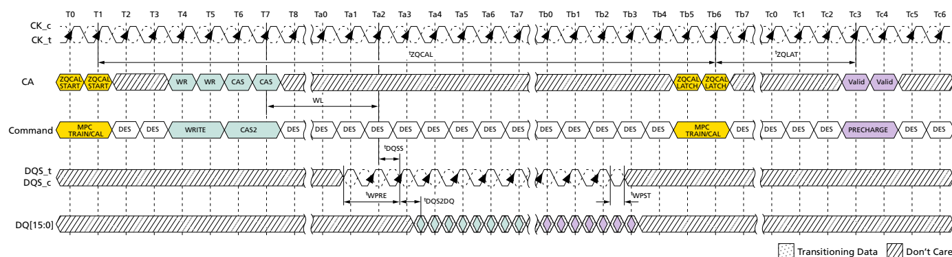
Figure 139: ZQCAL Timing
