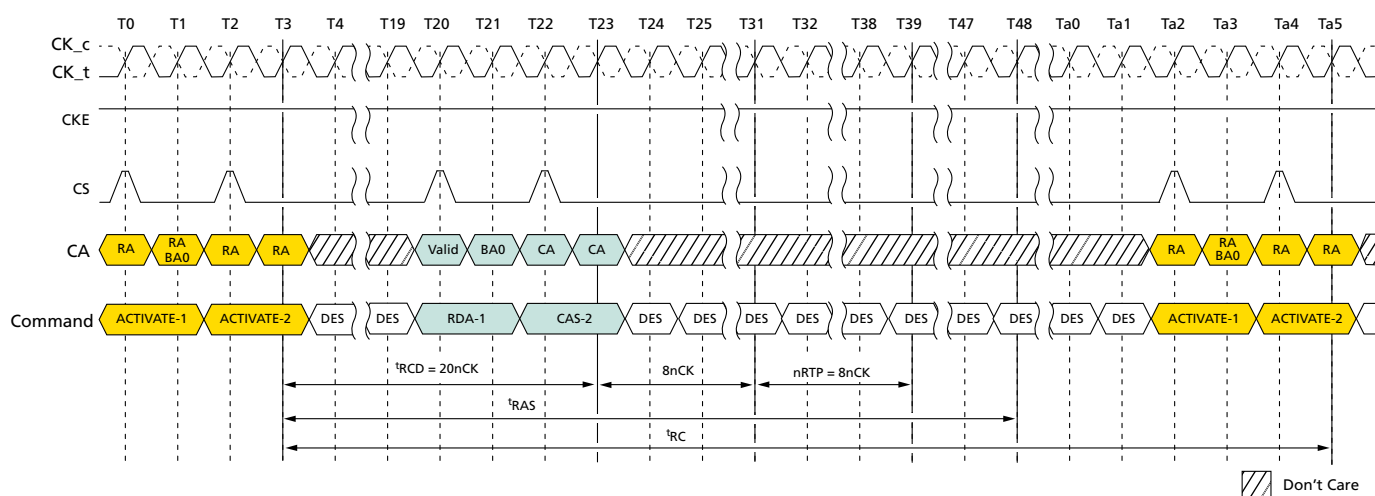
Figure 72: Command Input Timing with RAS Lock
