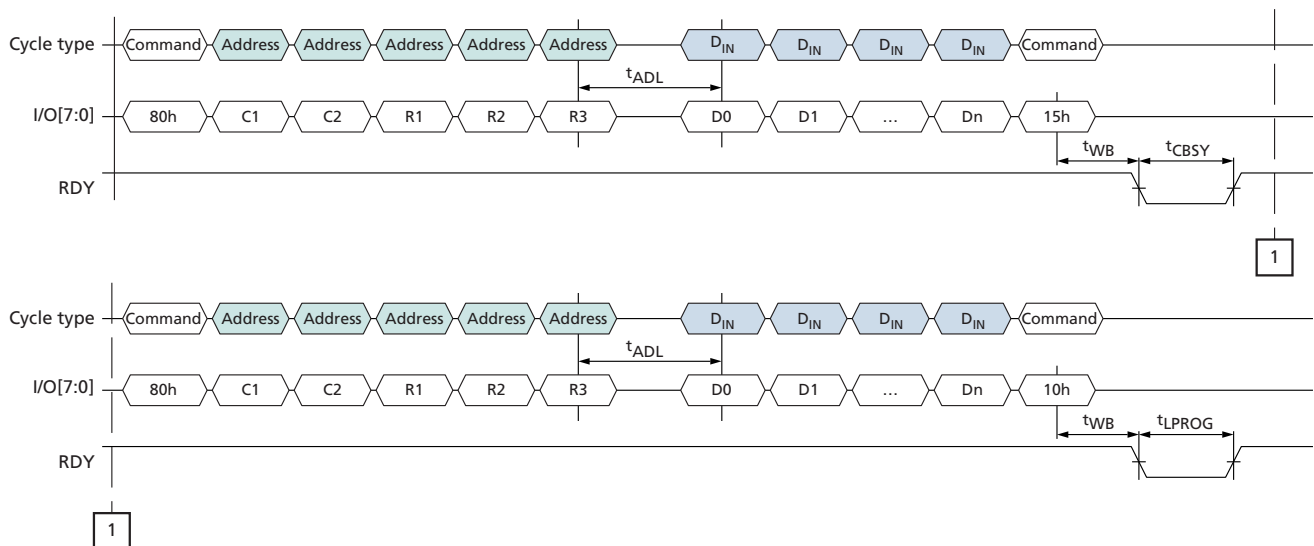
Figure 35: PROGRAM PAGE CACHE (80h–15h) Operation (End)
