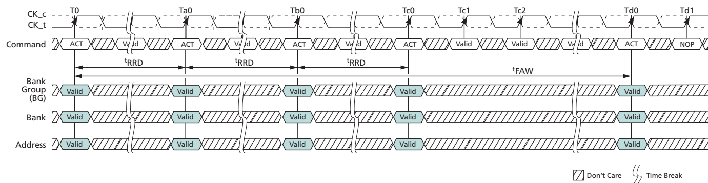
Figure 79: t_{FAW} Timing
