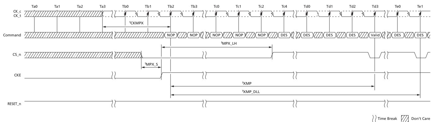
Figure 47: Maximum Power-Saving Mode Exit
