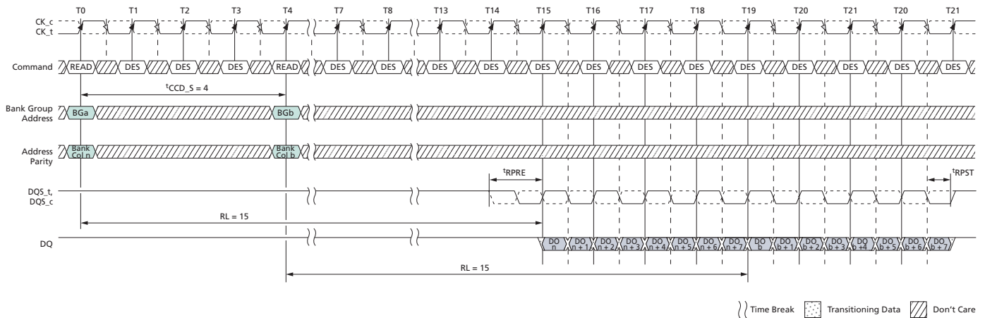
Figure 155: Consecutive READ (BL8) with 1 st CK Preamble and CA Parity in Different Bank Group
