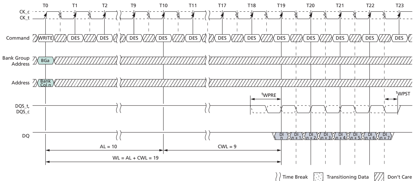
Figure 170: WRITE Burst Operation, WL = 19 (AL = 10, CWL = 9, BL8)
