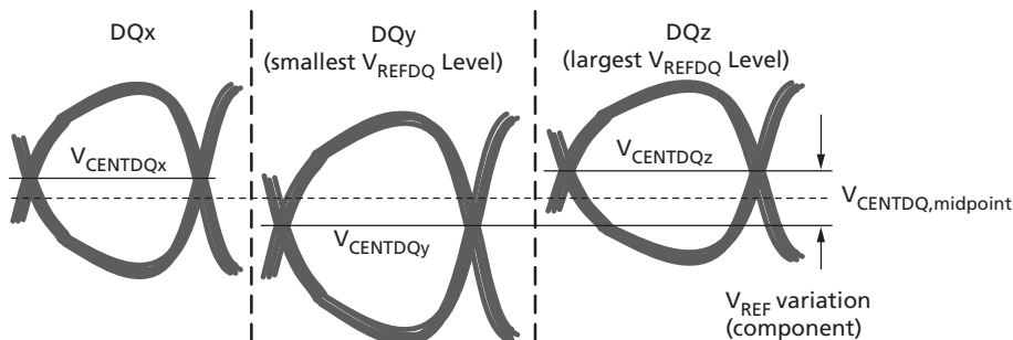
Figure 165: V_{\text{CENT\_DQ}} V_{\text{REFDQ}} Voltage Variation
