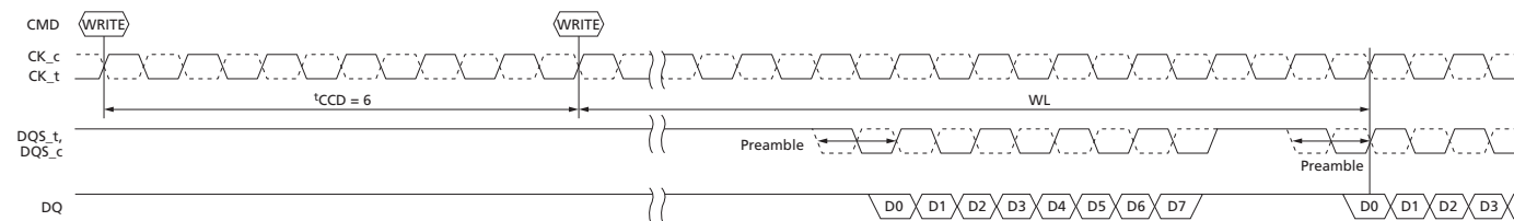
Figure 110: 1 t CK vs. 2 t CK WRITE Preamble Mode, t_{CCD} = 6
