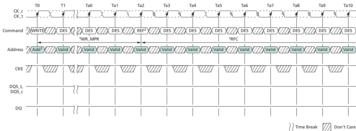
Figure 40: WRITE-to-REFRESH Timing
