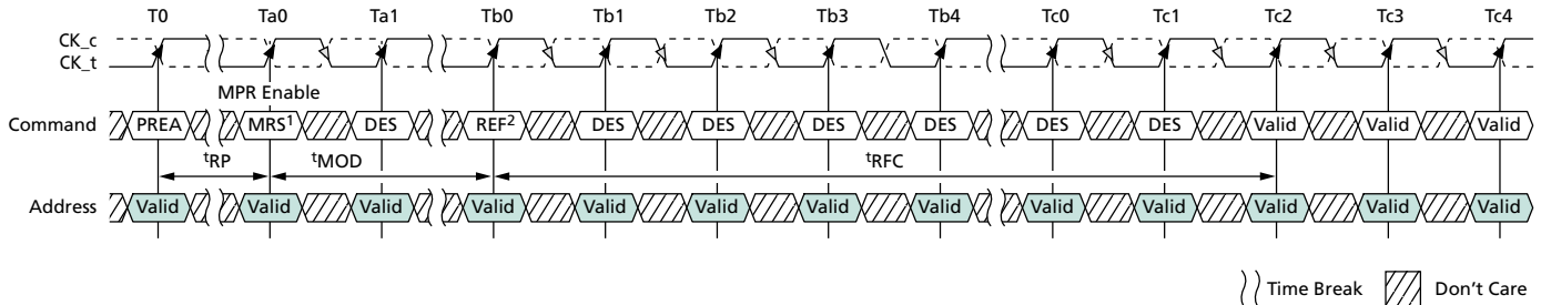
Figure 41: REFRESH Timing
