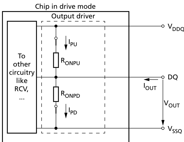
Figure 238: Output Driver: Definition of Voltages and Currents
