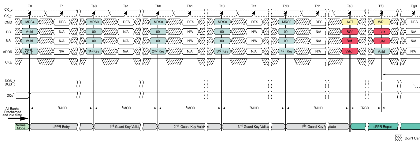
Figure 79: sPPR – Entry
