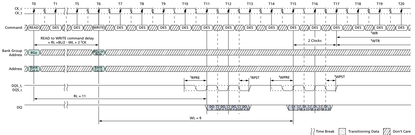
Figure 147: READ (BC4) Fixed to WRITE (BC4) Fixed with 1^t\text{CK} Preamble in Same or Different Bank Group
