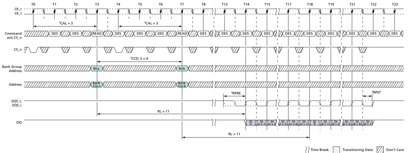
Figure 163: Consecutive READ (BL8) with CAL (3 t CK) and 1 t CK Preamble in Different Bank Group
