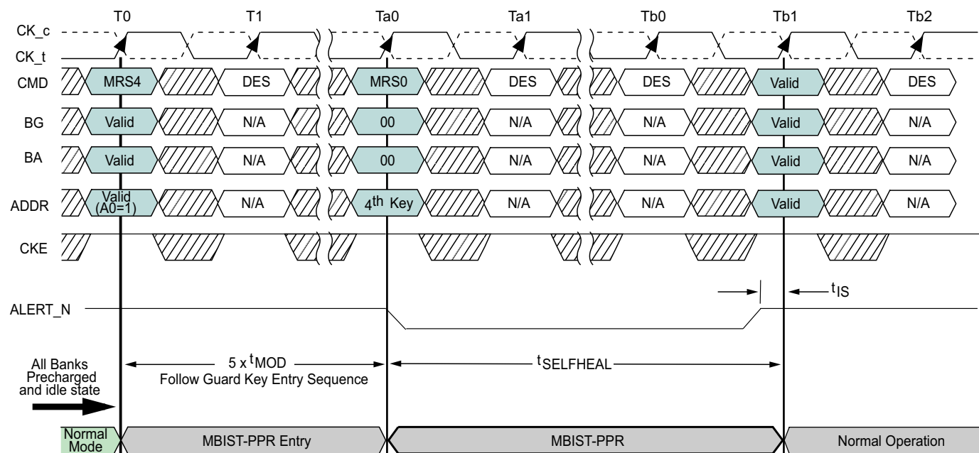
Figure 81: MBIST-PPR Sequence
