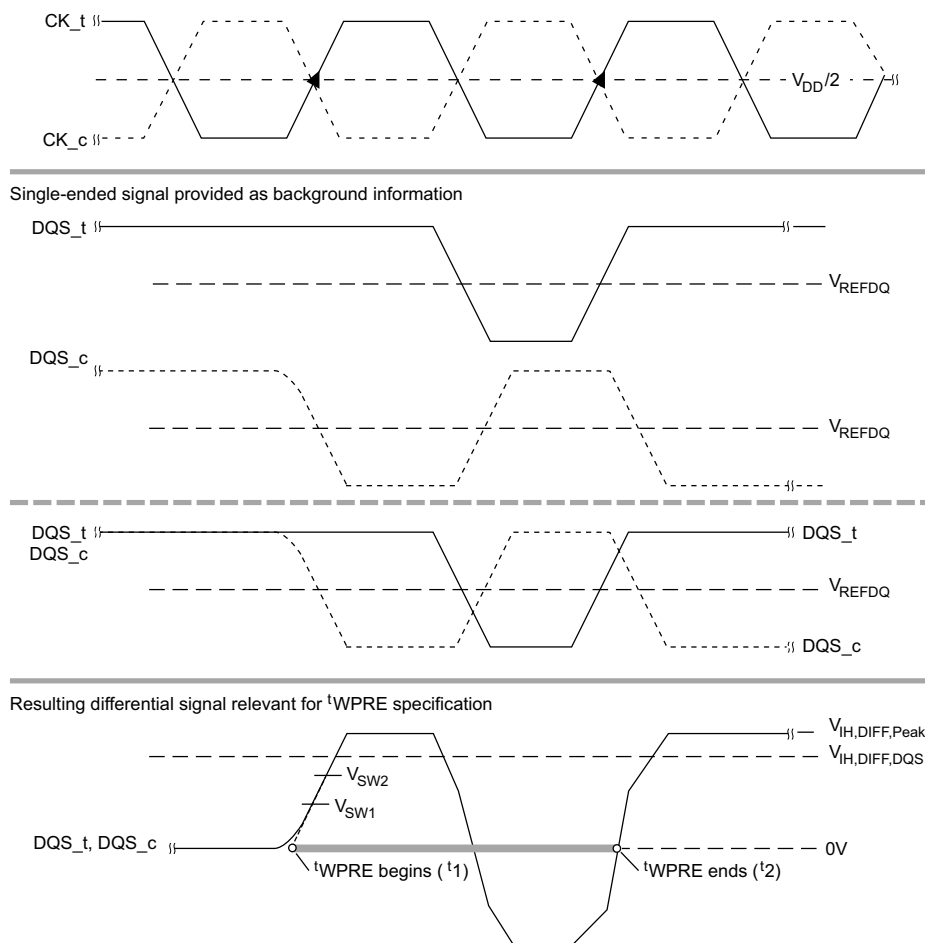
Figure 166: t_{\text{WPRE}} Method for Calculating Transitions and Endpoints
