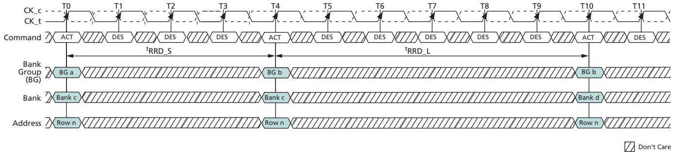
Figure 122: t_{RRD} Timing
