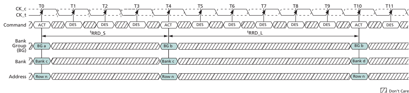
Figure 82: t_{RRD} Timing
