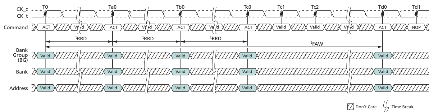
Figure 83: t_{FAW} Timing
