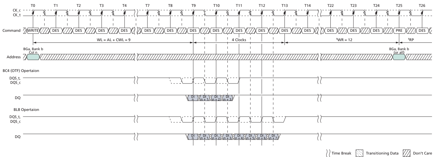
Figure 190: WRITE (BL8/BC4-OTF) to PRECHARGE with 1t_{CK} Preamble
