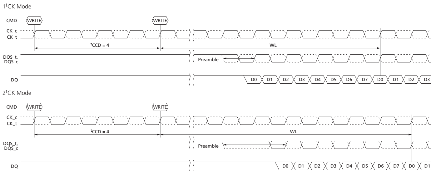
Figure 112: 1 t CK vs. 2 t CK WRITE Preamble Mode, t CCD = 4
