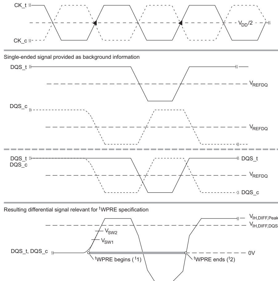
Figure 165: t WPRE Method for Calculating Transitions and Endpoints
