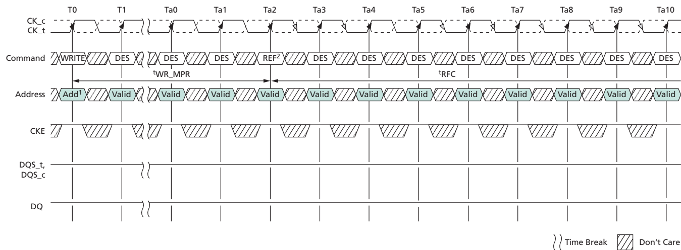
Figure 42: WRITE-to-REFRESH Timing
