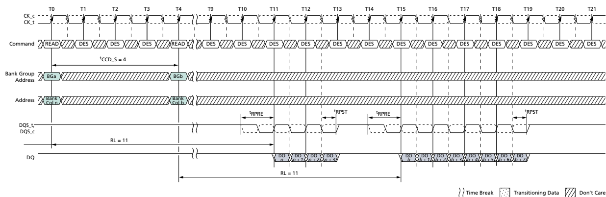
Figure 140: READ (BC4) to READ (BL8) OTF with 1 t CK Preamble in Different Bank Group
