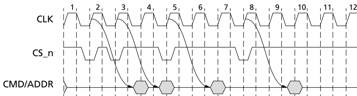
Figure 26: CAL Timing Example (Consecutive \text{CS}_n = \text{LOW} )
