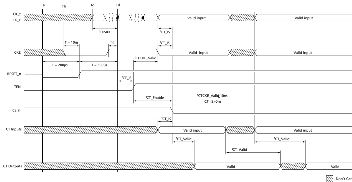
Figure 73: Connectivity Test Mode Entry
