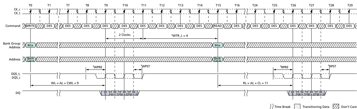
Figure 188: WRITE (BC4) Fixed to READ (BC4) Fixed with 1 st CK Preamble in Same Bank Group
