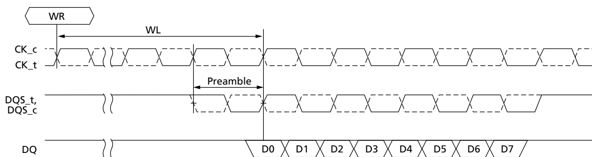
Figure 110: 1^t\text{CK} vs. 2^t\text{CK} WRITE Preamble Mode
