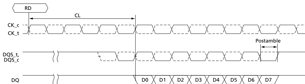
Figure 117: READ Postamble
