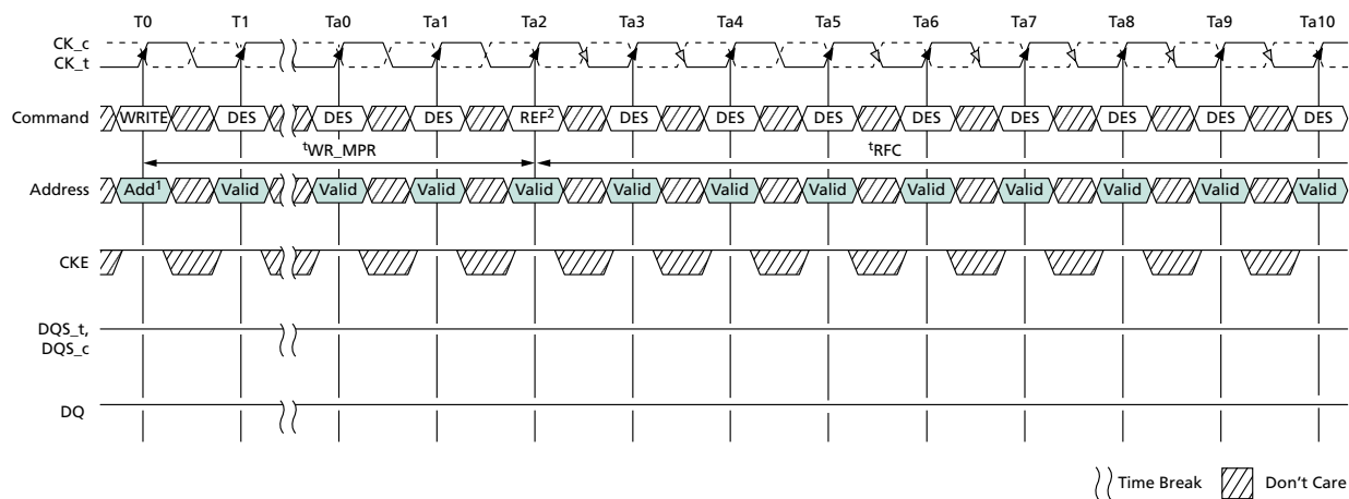
Figure 42: WRITE-to-REFRESH Timing
