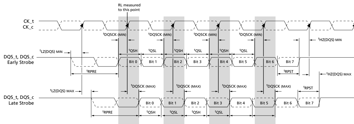
Figure 125: Clock-to-Data Strobe Relationship
