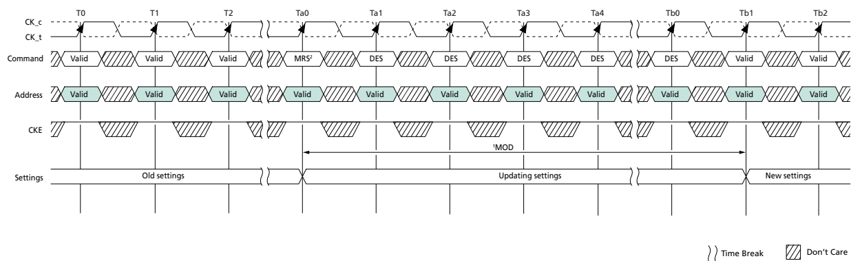
Figure 17: t_{MOD} Timing
