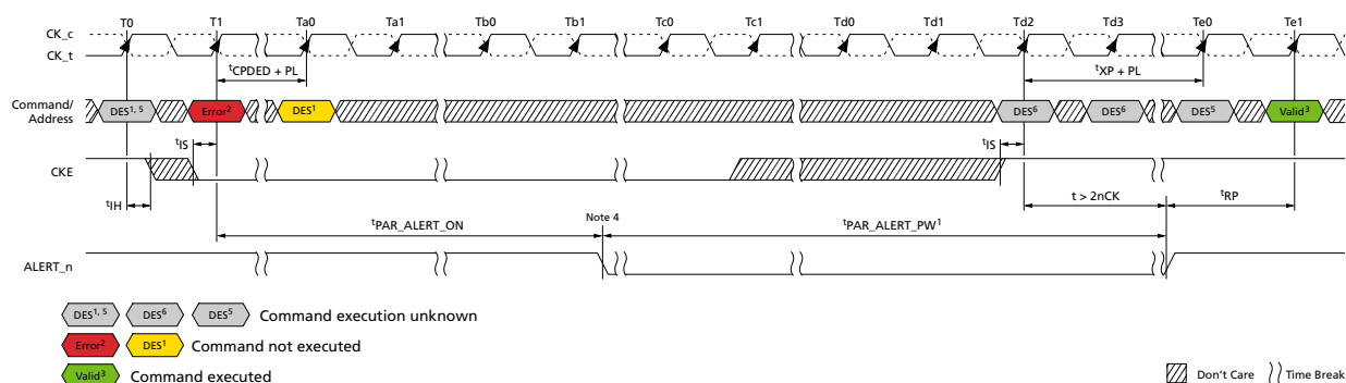
Figure 53: CA Parity Error Checking – SRE Attempt
