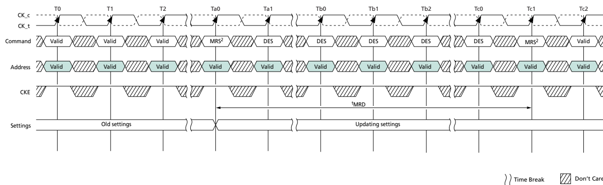
Figure 16: t_{MRD} Timing
