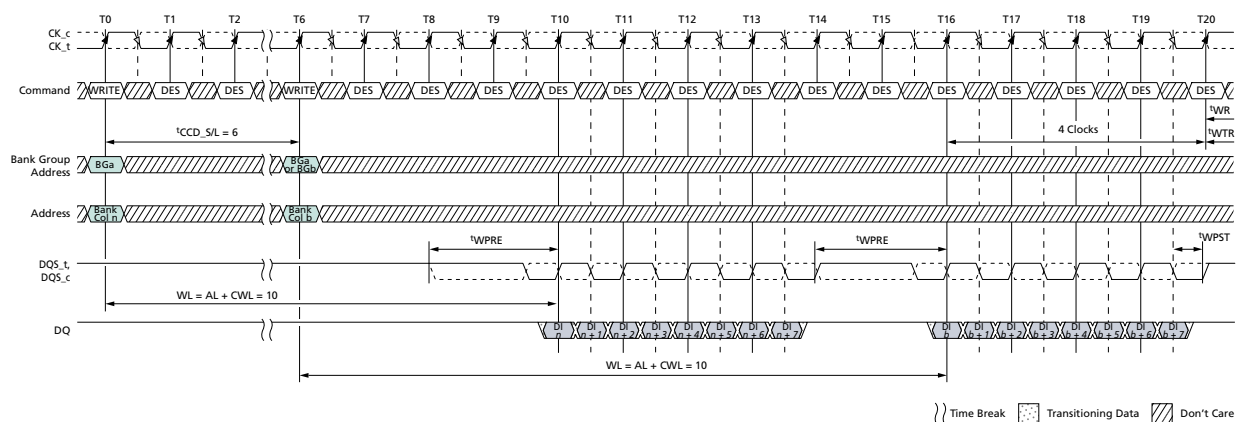
Figure 177: Nonconsecutive WRITE (BL8) with 2 t CK Preamble in Same or Different Bank Group
