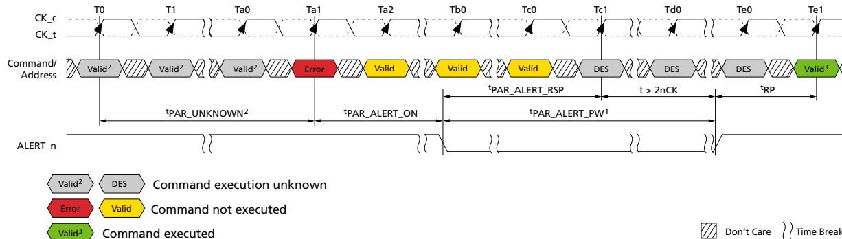
Figure 52: Persistent CA Parity Error Checking Operation
