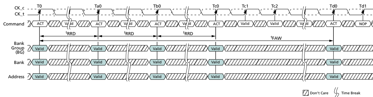
Figure 82: t_{FAW} Timing
