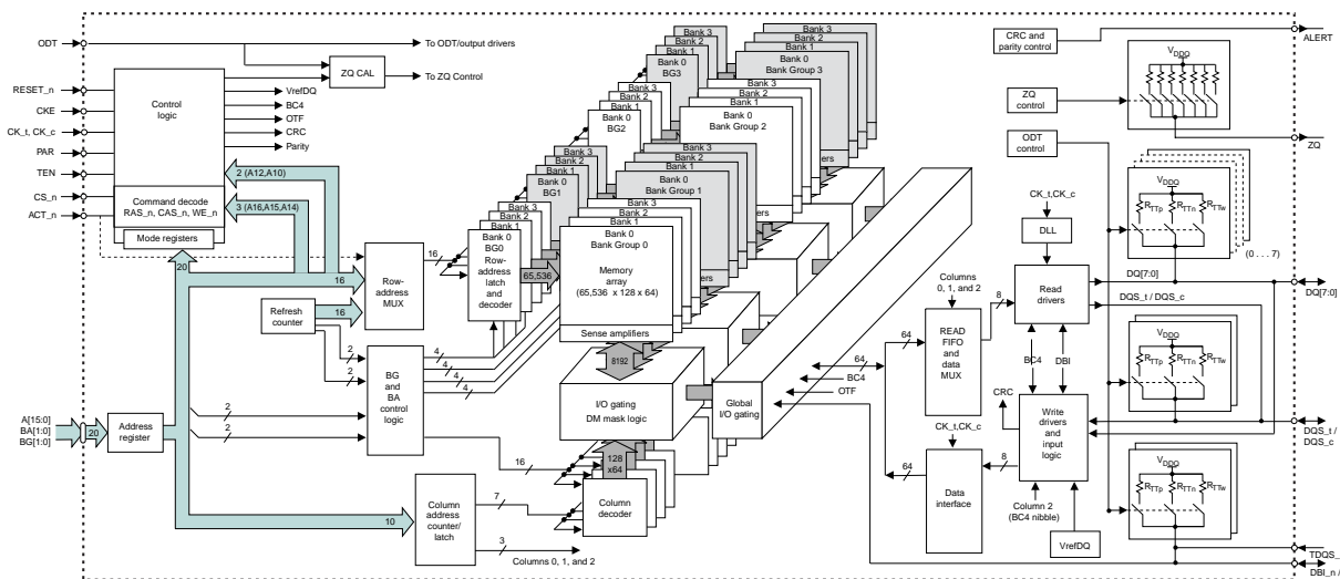
Figure 2: 1 Gig × 8 Functional Block Diagram
