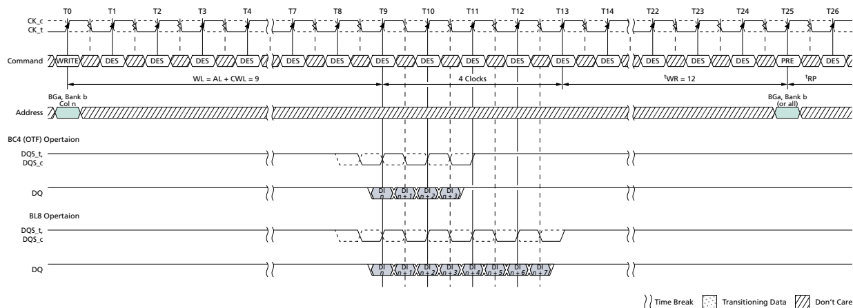
Figure 189: WRITE (BL8/BC4-OTF) to PRECHARGE with 1 st CK Preamble
