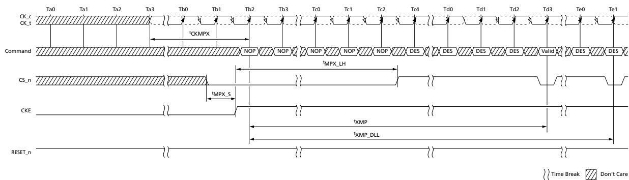
Figure 49: Maximum Power-Saving Mode Exit
