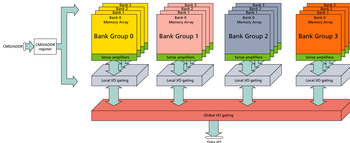
Figure 118: Bank Group x4/x8 Block Diagram
