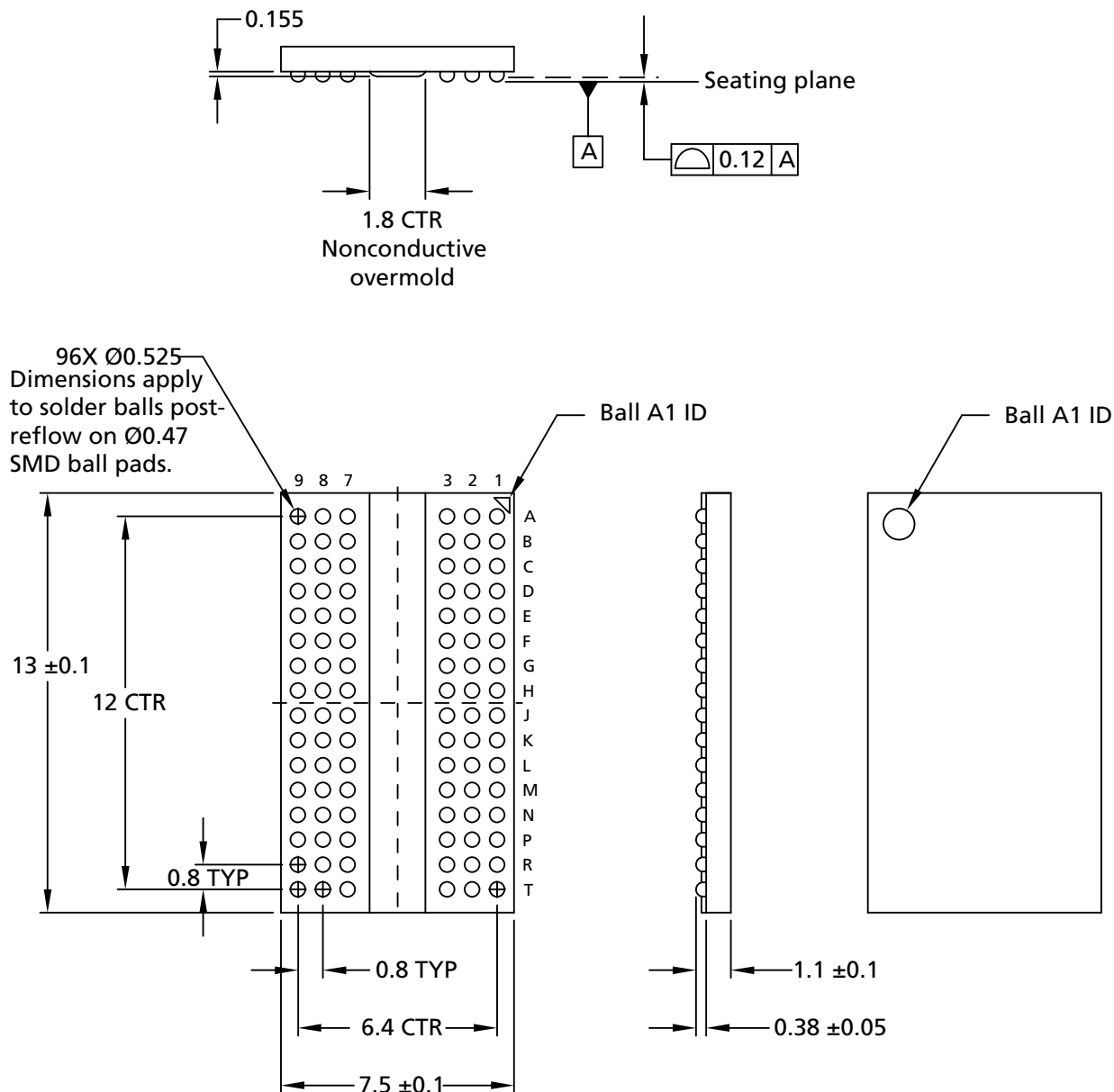
Figure 12: 96-Ball FBGA – x16 (TD)
