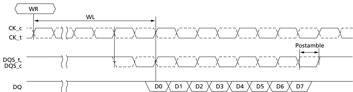
Figure 116: WRITE Postamble
