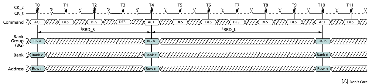
Figure 121: t_{RRD} Timing
