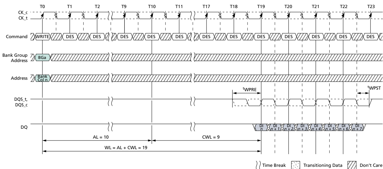
Figure 173: WRITE Burst Operation, WL = 19 (AL = 10, CWL = 9, BL8)
