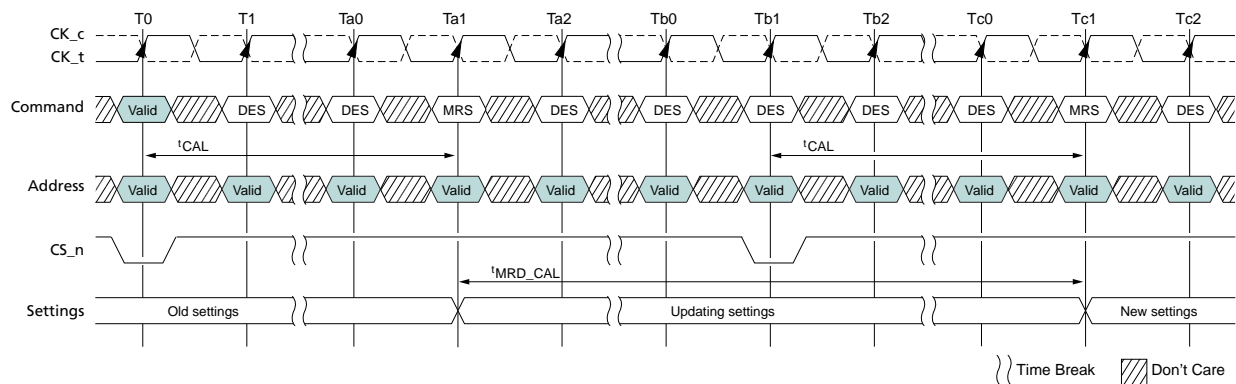
Figure 30: t^{\text{MRD\_CAL}} , Mode Register Cycle Time With CAL Enabled
