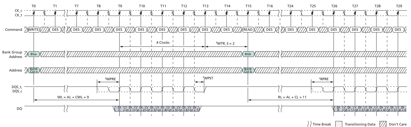
Figure 183: WRITE (BL8) to READ (BL8) with 1^{\text{t}} CK Preamble in Different Bank Group
