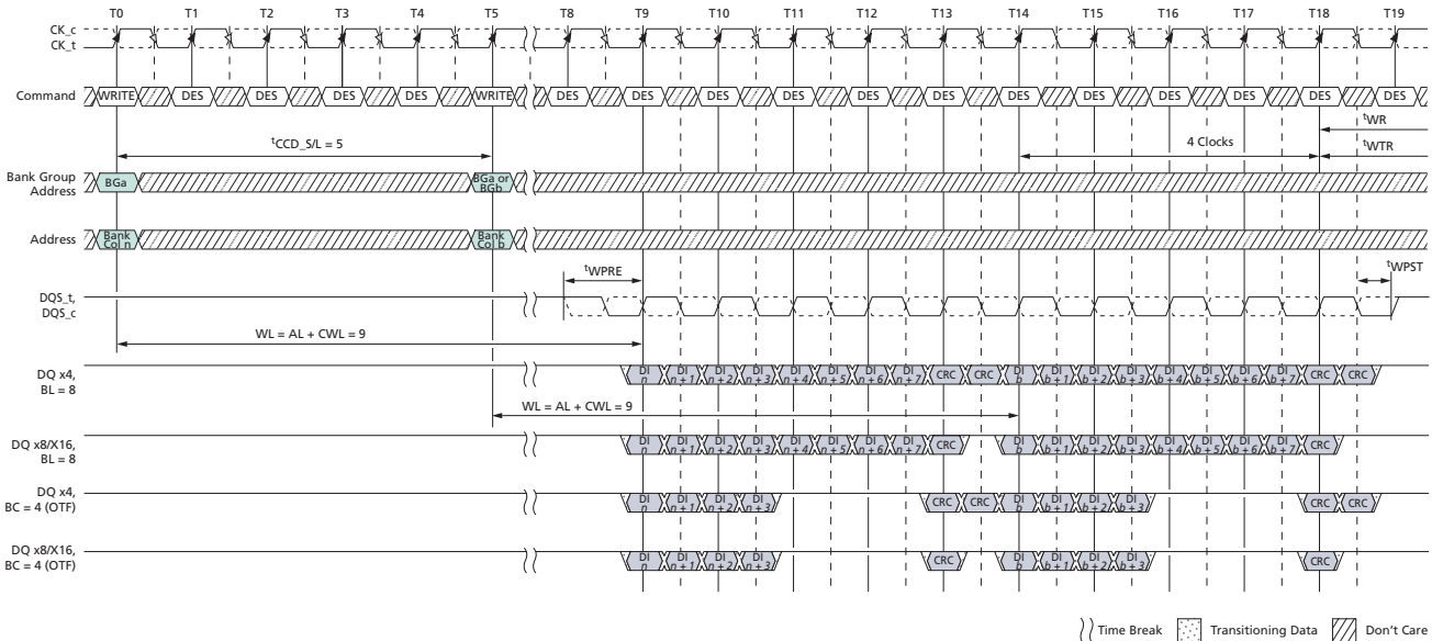
Figure 196: Consecutive WRITE (BL8/BC4-OTF) with 1^{\text{st}} CK Preamble and Write CRC in Same or Different Bank Group
