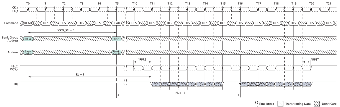
Figure 134: Nonconsecutive READ (BL8) with 1^t\text{CK} Preamble in Same or Different Bank Group
