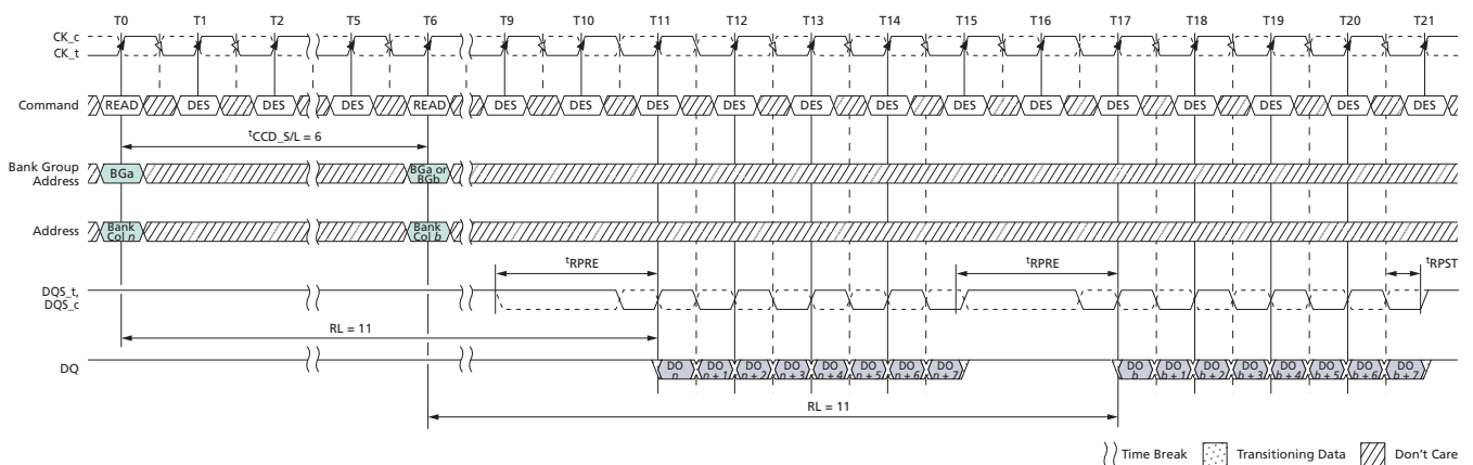
Figure 135: Nonconsecutive READ (BL8) with 2^t\text{CK} Preamble in Same or Different Bank Group
