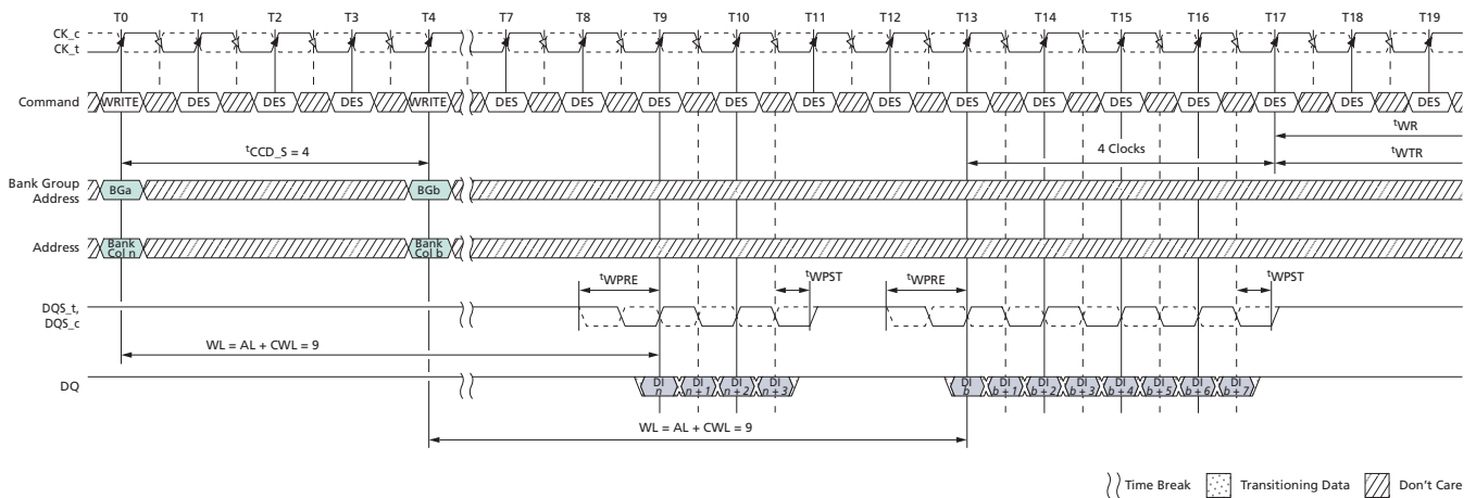
Figure 182: WRITE (BC4) OTF to WRITE (BL8) with 1^{\text{t}} CK Preamble in Different Bank Group
