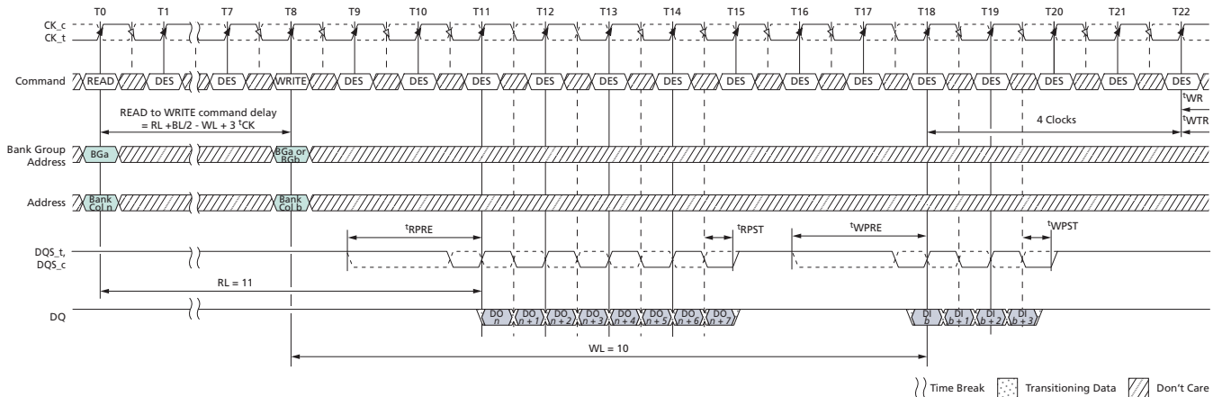
Figure 151: READ (BL8) to WRITE (BC4) OTF with 2^t\text{CK} Preamble in Same or Different Bank Group
