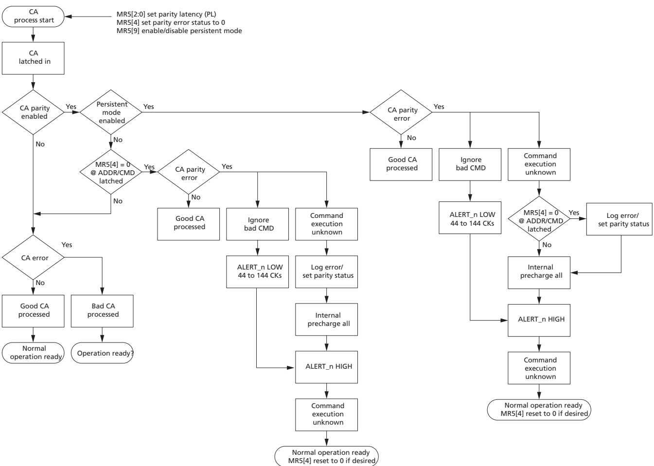
Figure 60: CA Parity Flow Diagram
