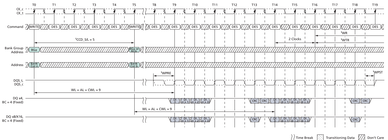
Figure 197: Consecutive WRITE (BC4-Fixed) with 1^{\text{st}} CK Preamble and Write CRC in Same or Different Bank Group
