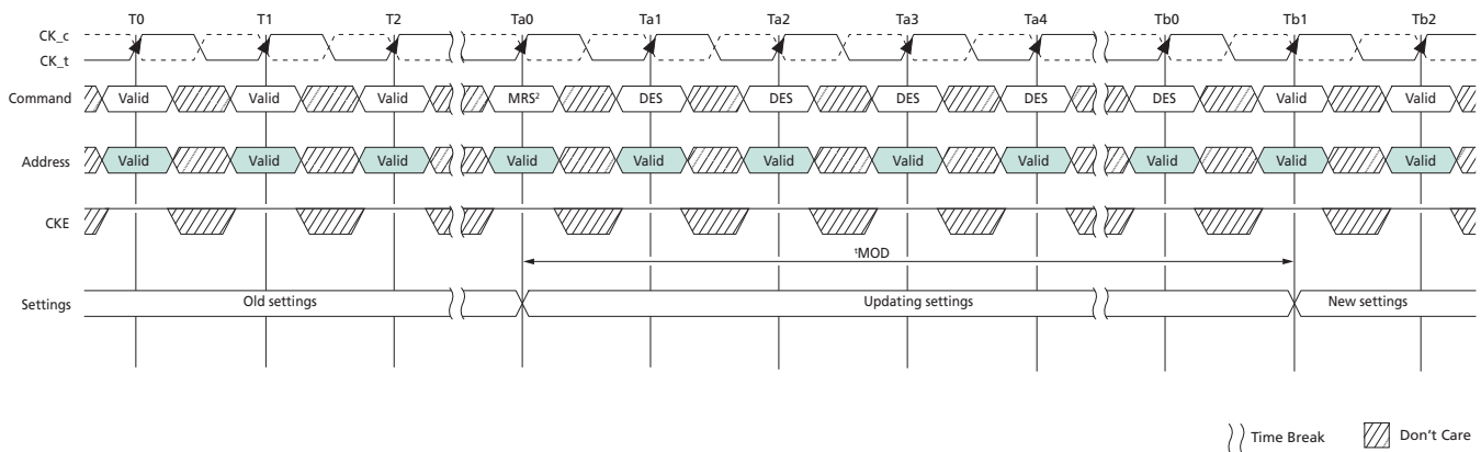
Figure 17: t^{\text{MOD}} Timing
