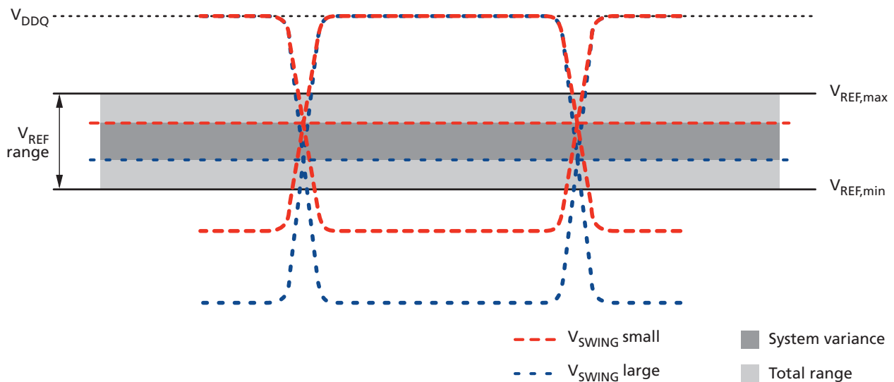
Figure 64: V_{\text{REFDQ}} Voltage Range
