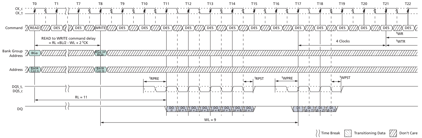
Figure 150: READ (BL8) to WRITE (BC4) OTF with 1^t\text{CK} Preamble in Same or Different Bank Group
