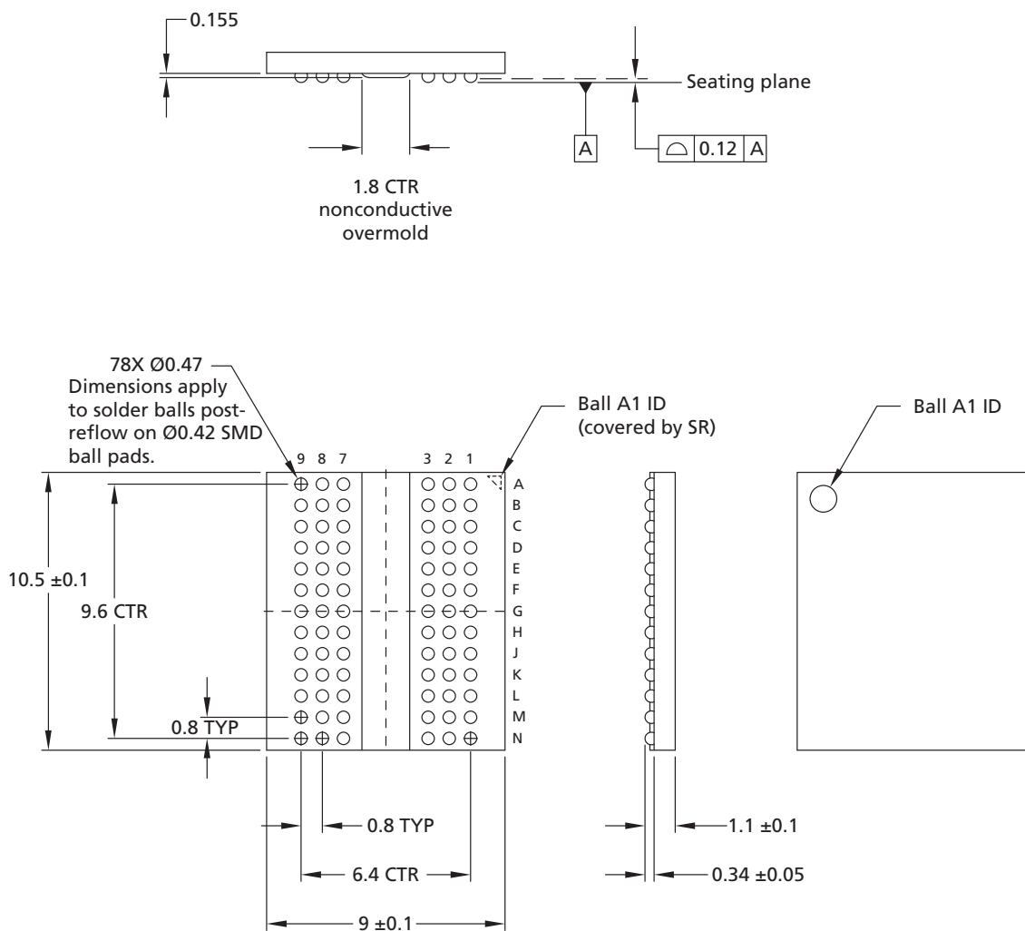
Figure 6: 78-Ball FBGA – x4, x8, "RH"
