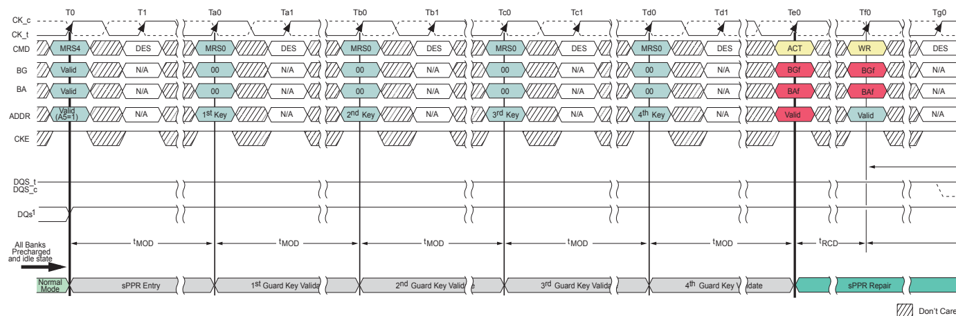
Figure 75: sPPR – Entry
