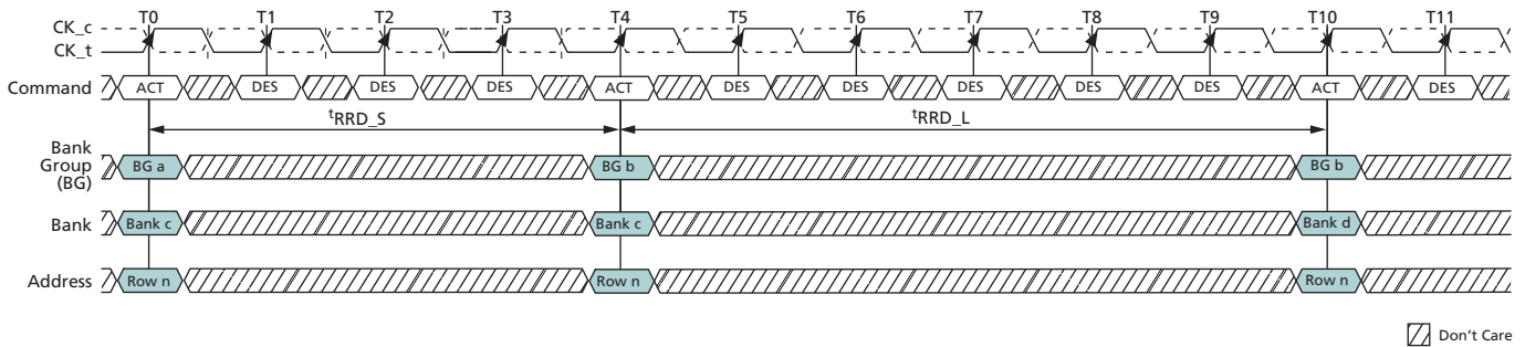
Figure 77: t_{RRD} Timing
