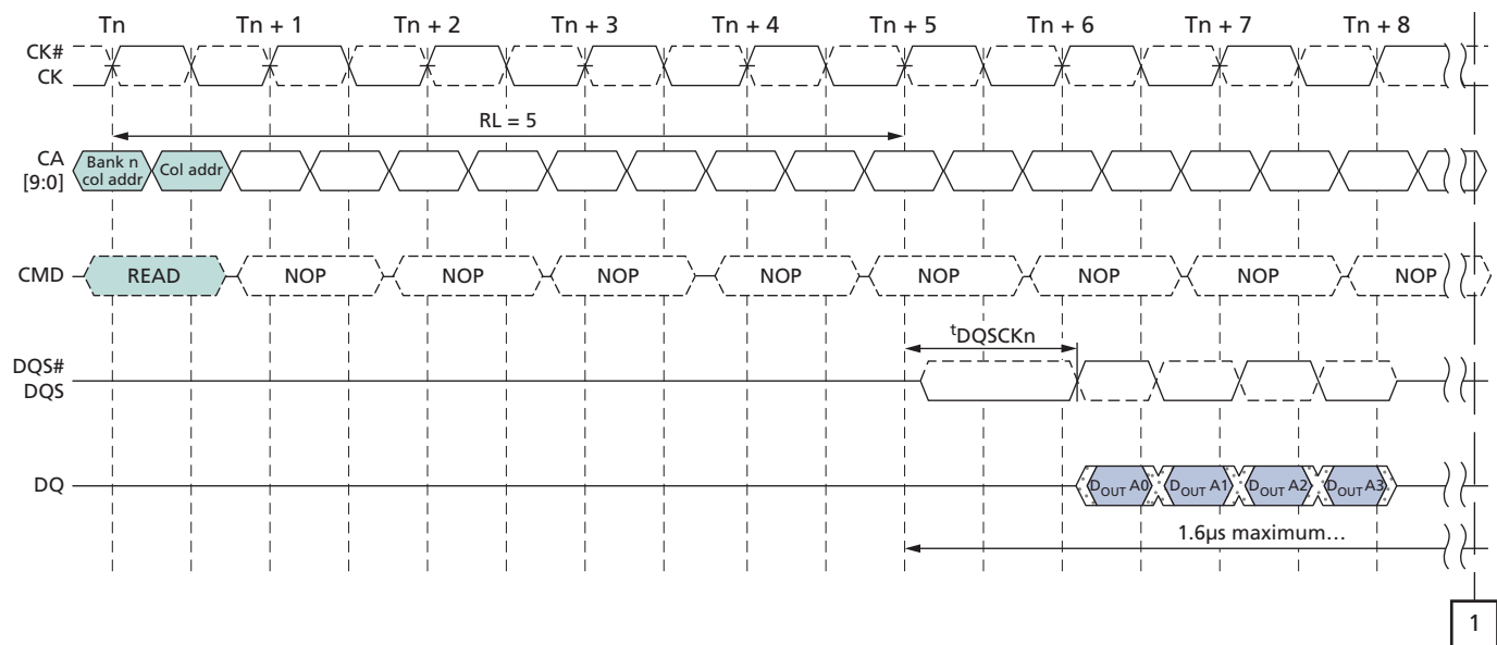
Figure 22: t_{DQCKDM} Timing
