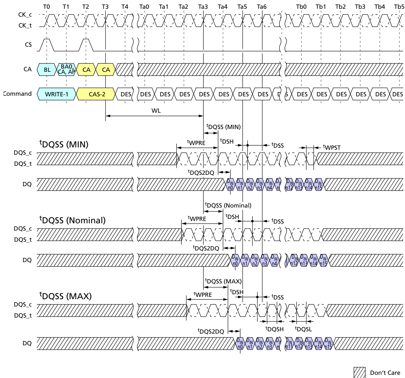
Figure 28: Write Timing
