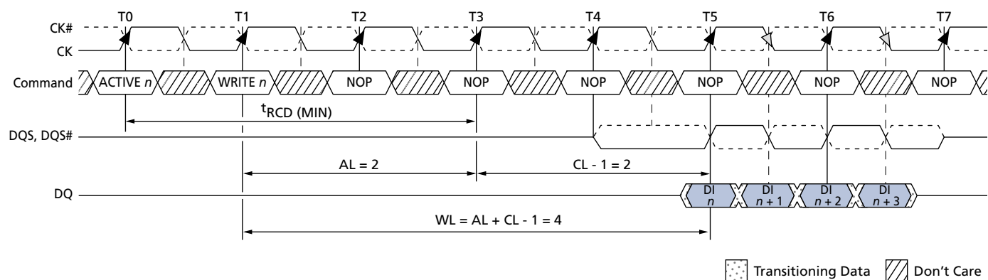
Figure 37: WRITE Latency
