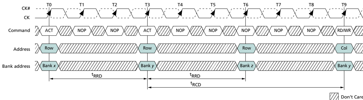
Figure 41: Example: Meeting t_{RRD} (MIN) and t_{RCD} (MIN)
