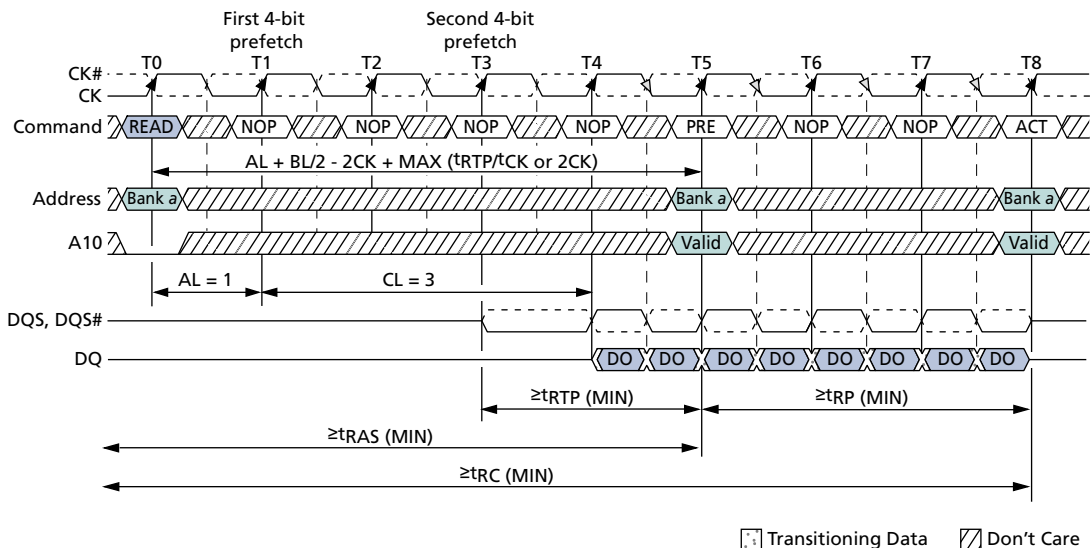
Figure 49: READ-to-PRECHARGE – BL = 8
