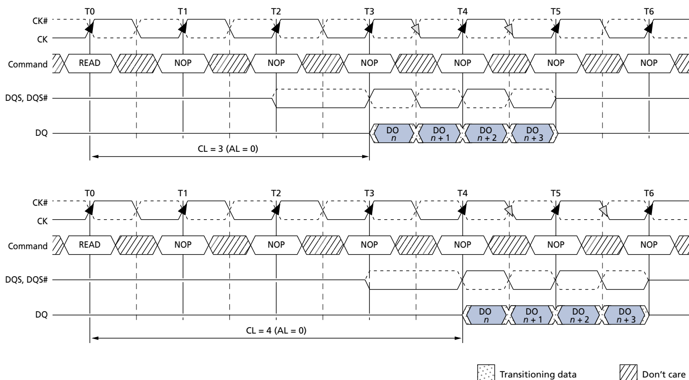
Figure 34: CL
