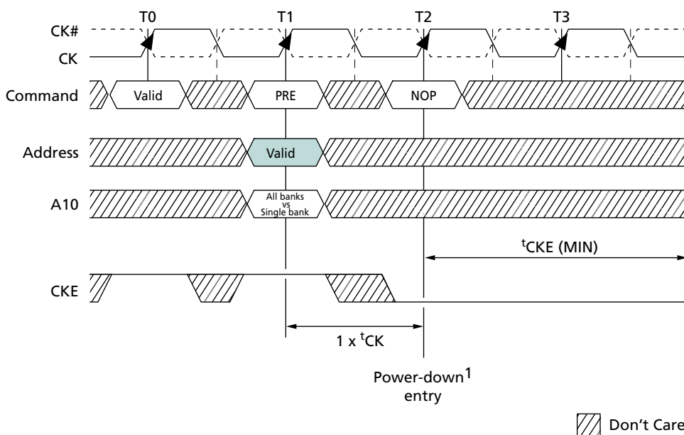
Figure 74: PRECHARGE Command-to-Power-Down Entry
