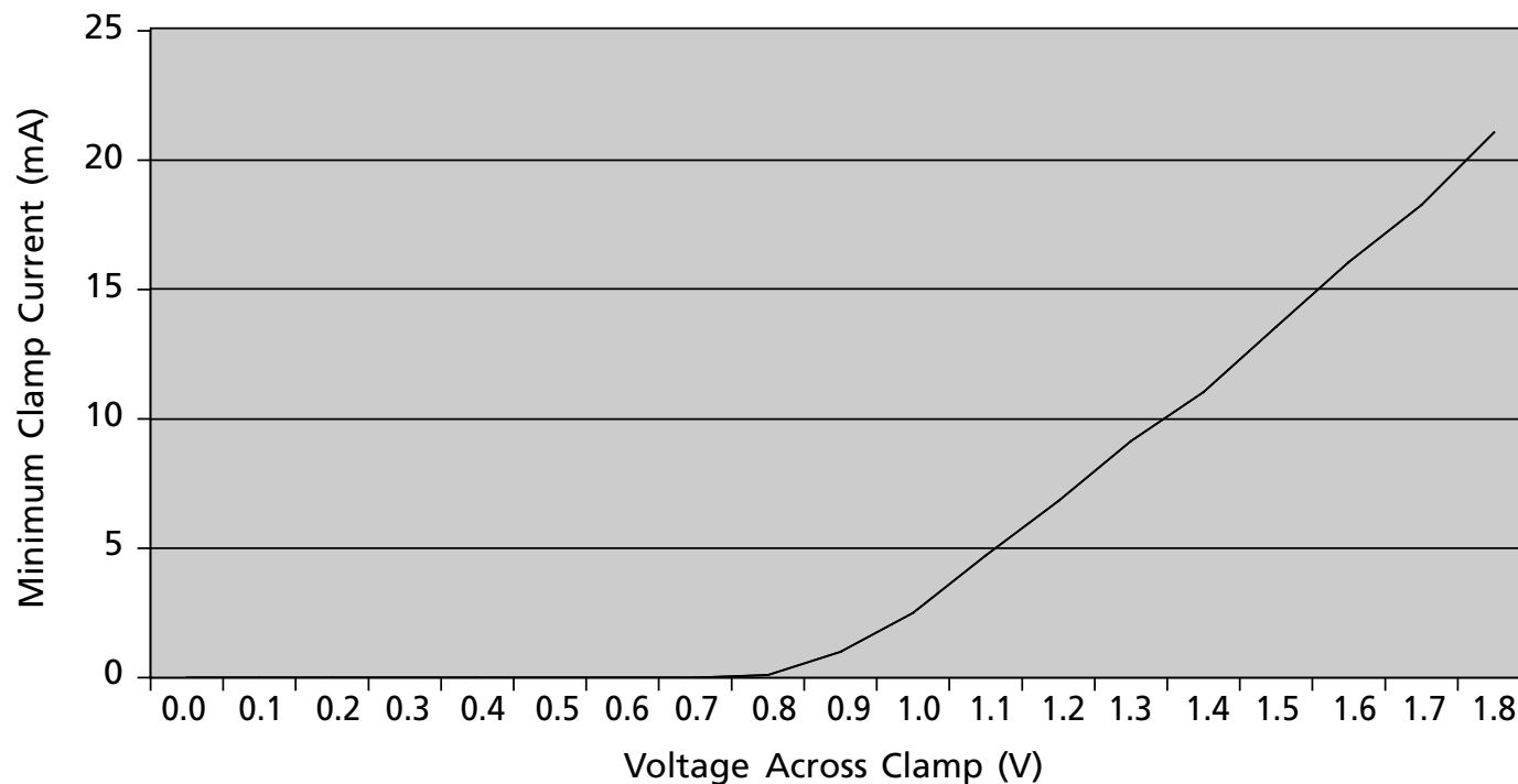
Figure 18: Input Clamp Characteristics
