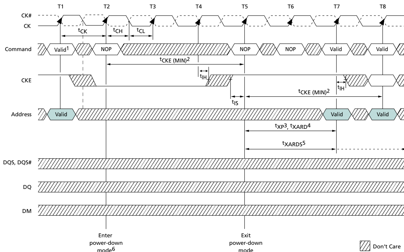
Figure 67: Power-Down
