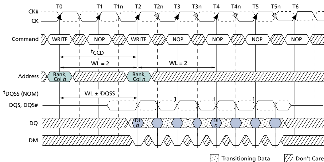
Figure 56: Consecutive WRITE-to-WRITE
