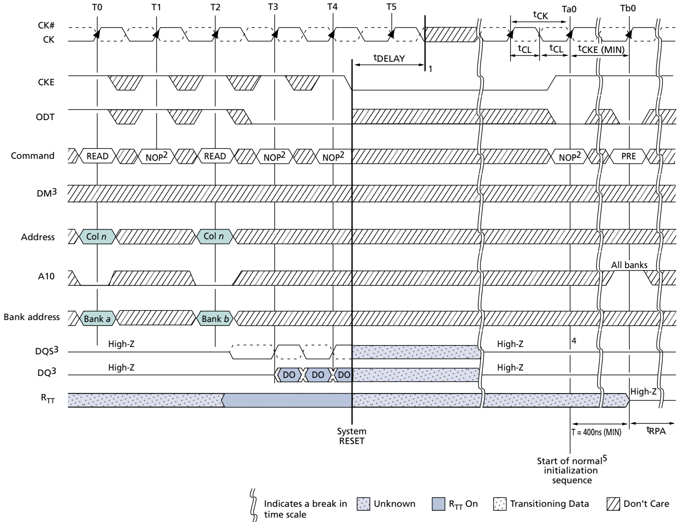
Figure 77: RESET Function
