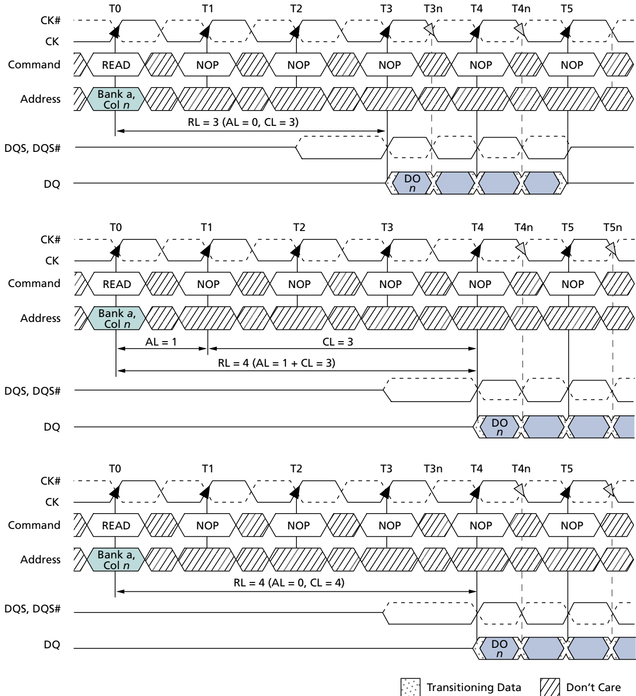
Figure 43: READ Latency
