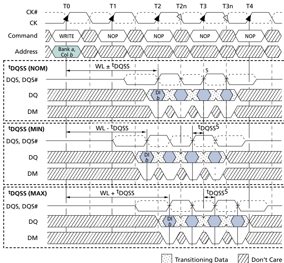
Figure 55: Write Burst
