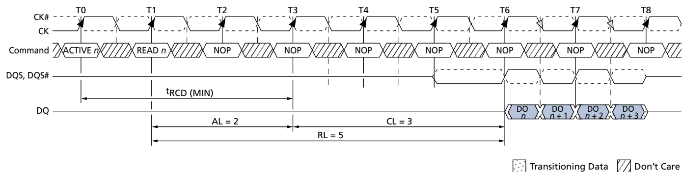
Figure 36: READ Latency
