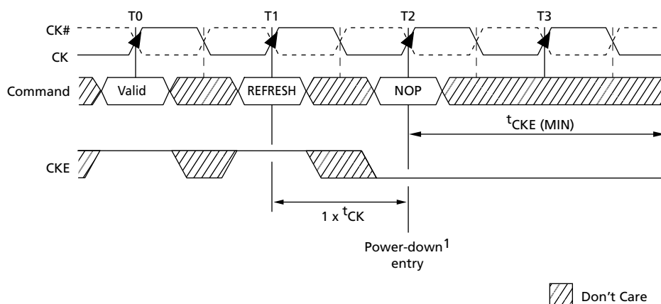
Figure 72: REFRESH Command-to-Power-Down Entry
