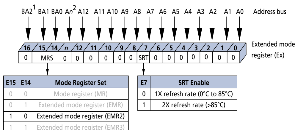
Figure 38: EMR2 Definition
