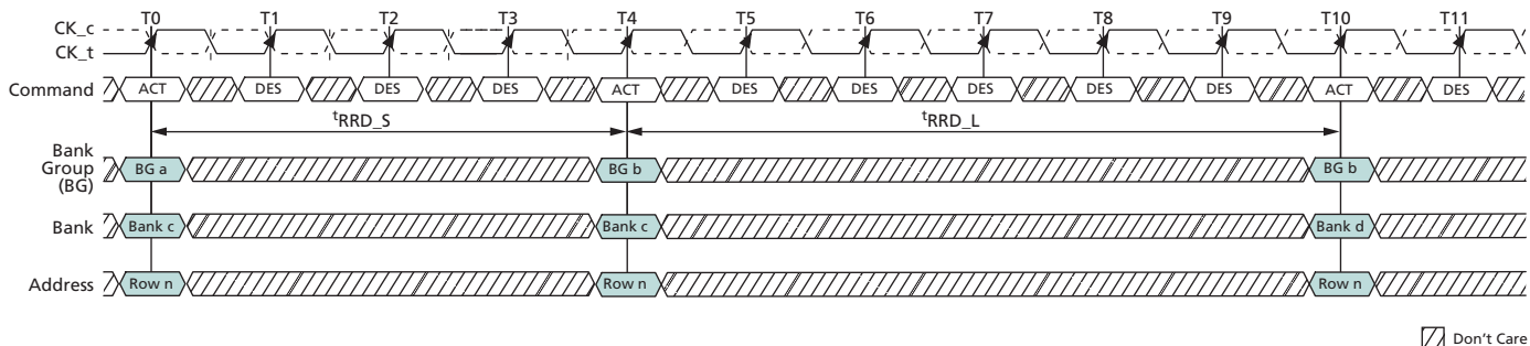
Figure 118: t_{RRD} Timing
