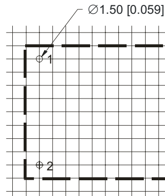
Top View PCB LAYOUT
