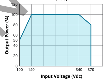
INPUT VOLTAGE DERATING CURVE (Vdc)
