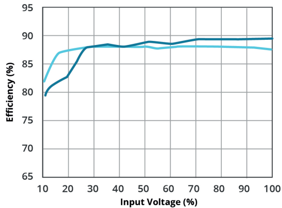
EFFICIENCY VS INPUT LOAD VOF-80B-15
