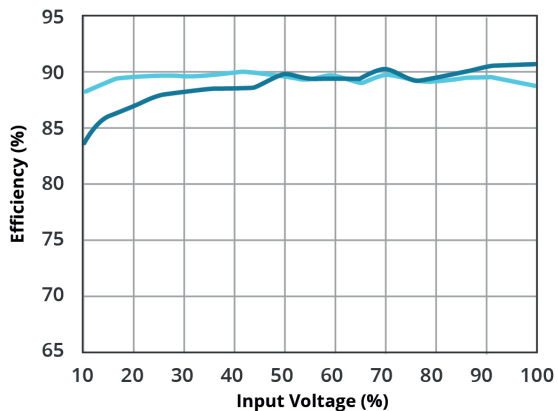
EFFICIENCY VS INPUT LOAD VOF-80B-48
