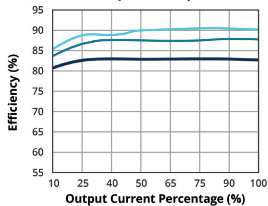
EFFICIENCY VS OUTPUT LOAD (at 230 Vac)
