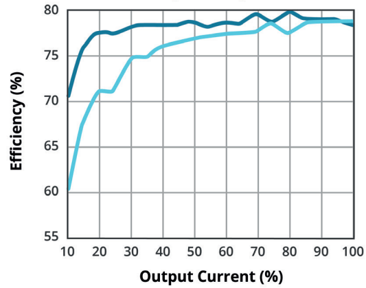
EFFICIENCY VS OUTPUT LOAD (VOF-4-15)
