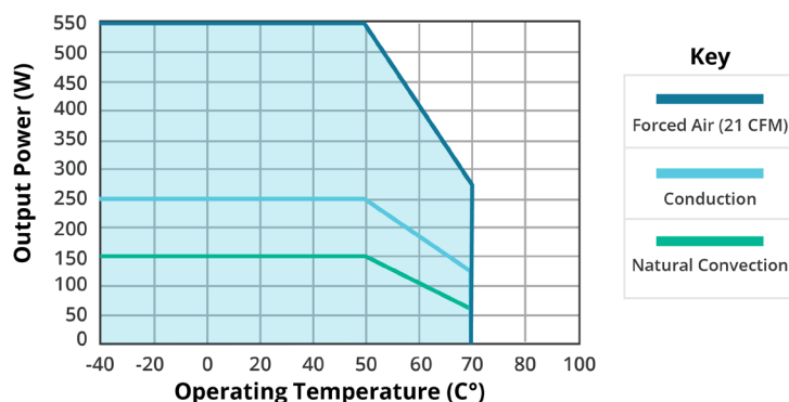
TEMPERATURE DERATING CURVE (all other output models)
