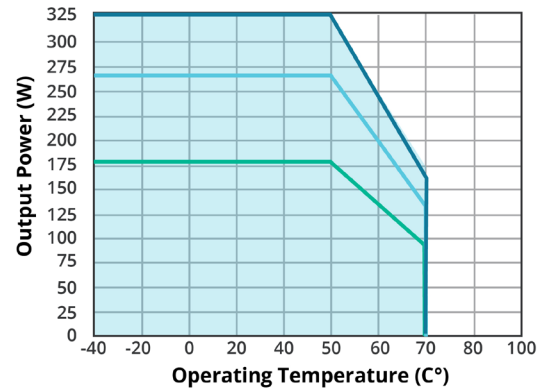
TEMPERATURE DERATING CURVE (15 Vdc output models)
