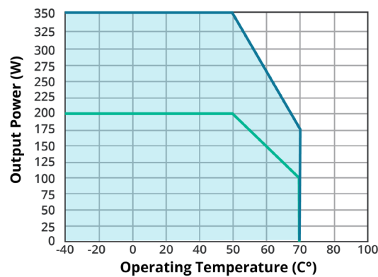
TEMPERATURE DERATING CURVE (all other output models)
