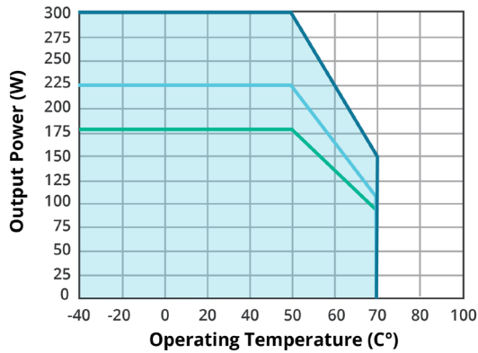
TEMPERATURE DERATING CURVE (12 Vdc output models)
