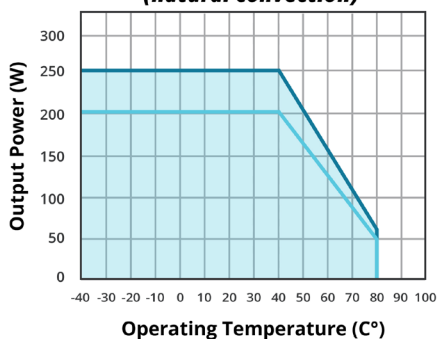
TEMPERATURE DERATING CURVE VMS-300A (natural convection)
