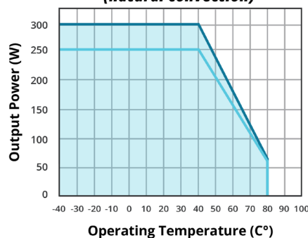
TEMPERATURE DERATING CURVE VMS-300A-CNF (natural convection)
