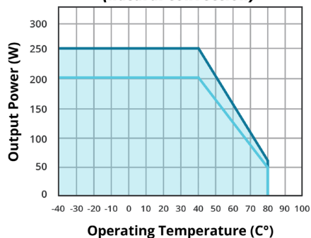
TEMPERATURE DERATING CURVE VMS-300A (natural convection)
