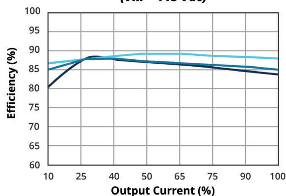
EFFICIENCY VS OUTPUT LOAD (Vin = 115 Vac)
