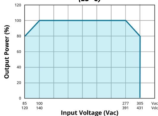
INPUT VOLTAGE DERATING CURVE (25 °C)
