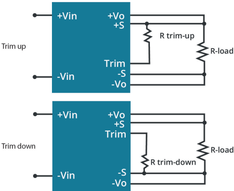
Application Circuit for Trim pin
