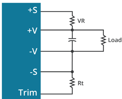
Figure 5 External Resistors
