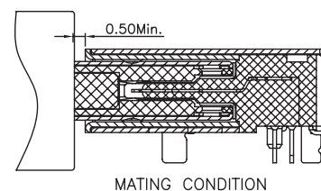
MATING CONDITION
