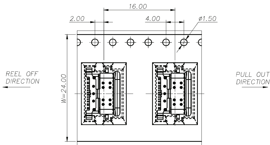
DETAIL X
