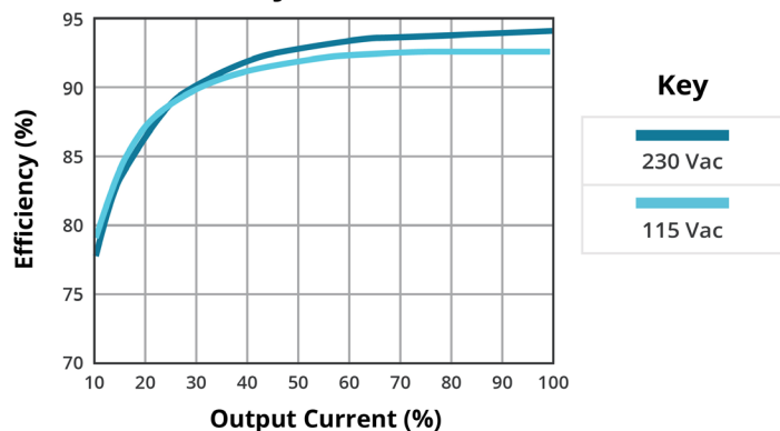
EFFICIENCY VS OUTPUT LOAD TJ-100-12
