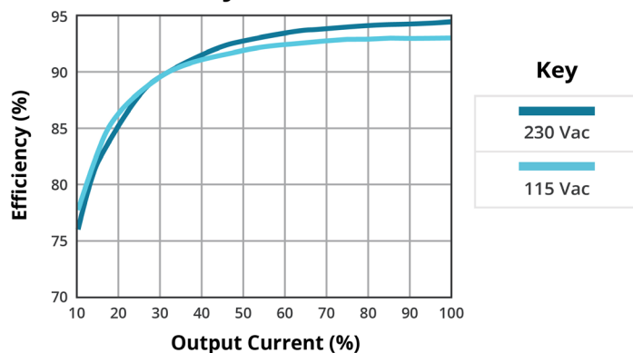
EFFICIENCY VS OUTPUT LOAD TJ-100-36
