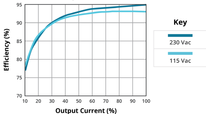
EFFICIENCY VS OUTPUT LOAD TJ-100-48
