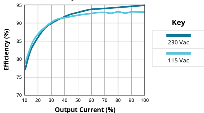
EFFICIENCY VS OUTPUT LOAD TJ-100-28
