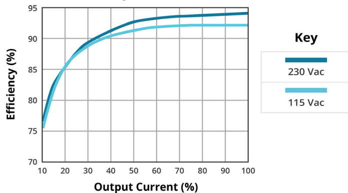
EFFICIENCY VS OUTPUT LOAD TJ-100-24
