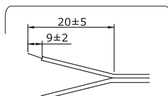
Stripped & Tinned
